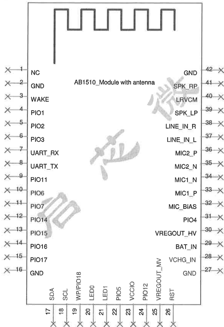
Figure 2-1 Pin Definition
