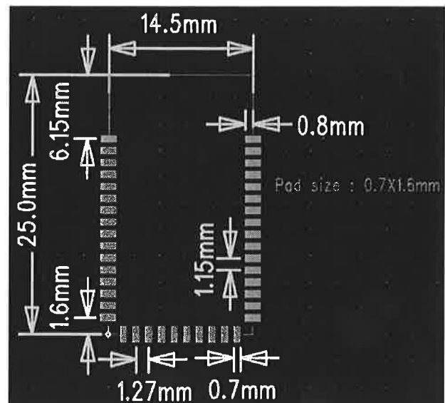
Figure 2-3 Module PCB footprint dimensions
