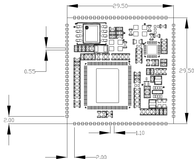
Figure 4. IDO-SOM2D01 dimensions
