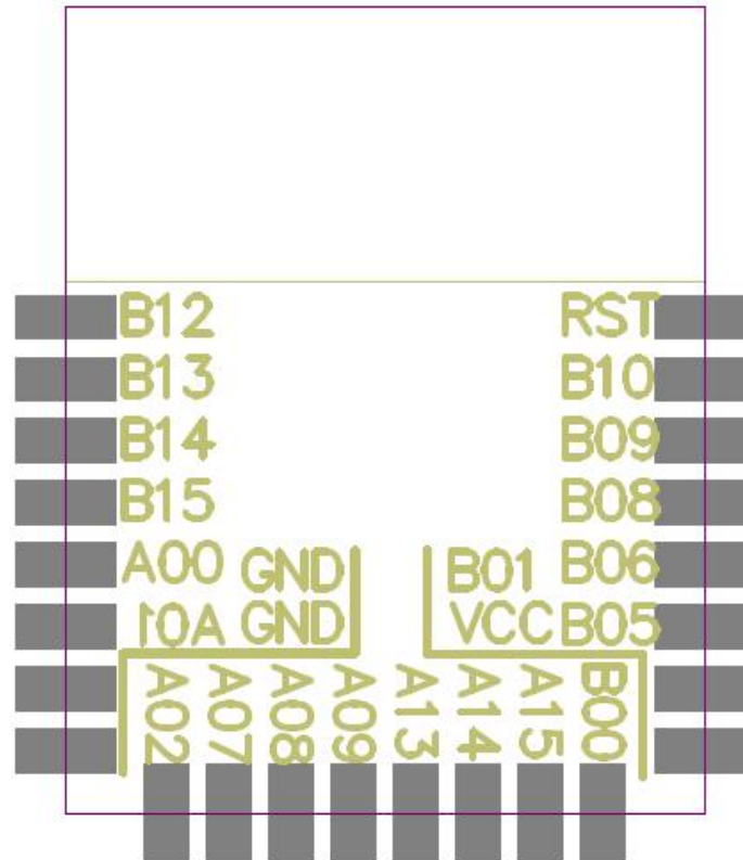
Figure 2 Top View
