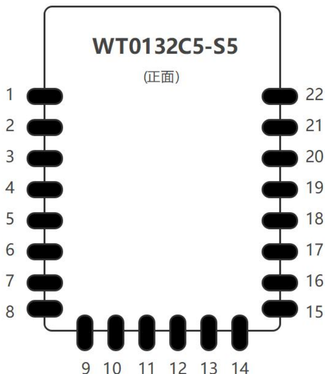
Figure 7: WT0132C5-S5 Pin Layout
