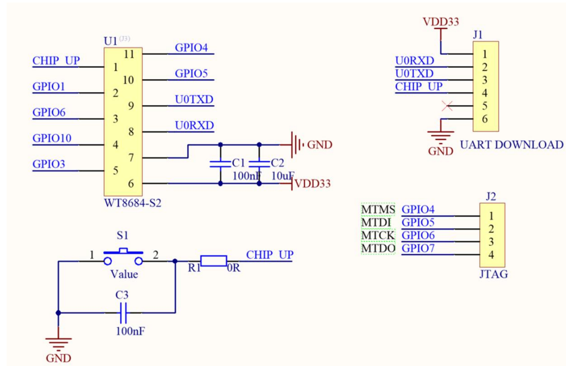
Figure 7 Peripheral Schematics
