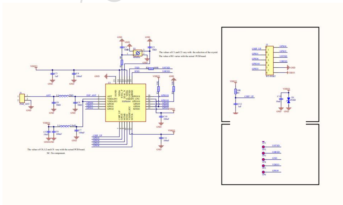
Figure 6 Module Schematics
