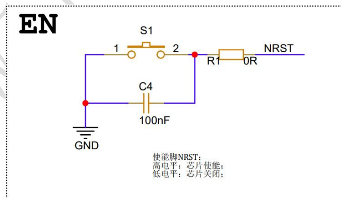
Figure 4 Button reset reference design
