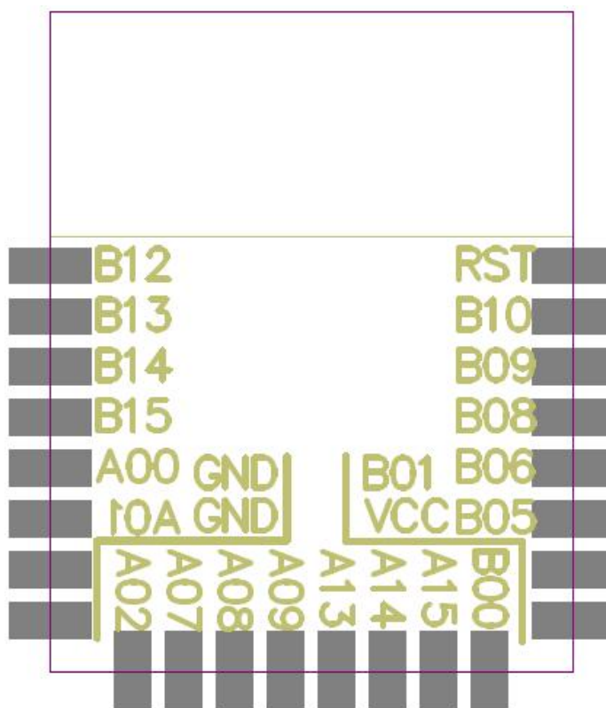
Figure 2 Top View of Pin Layout
