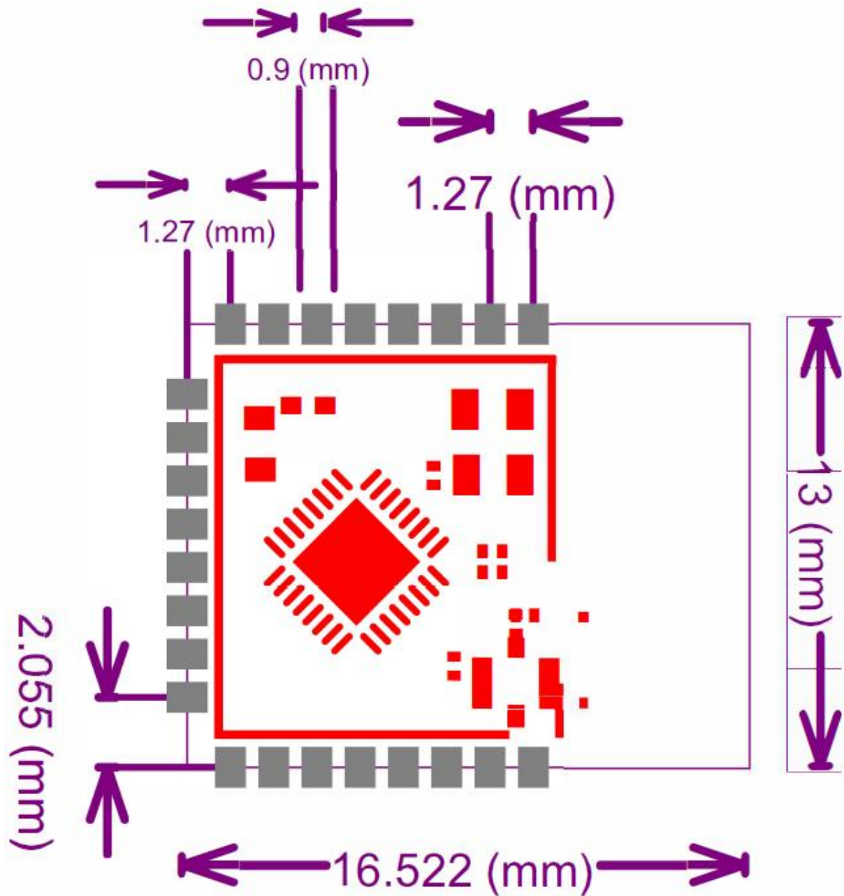
Figure 1 Module Dimensions
