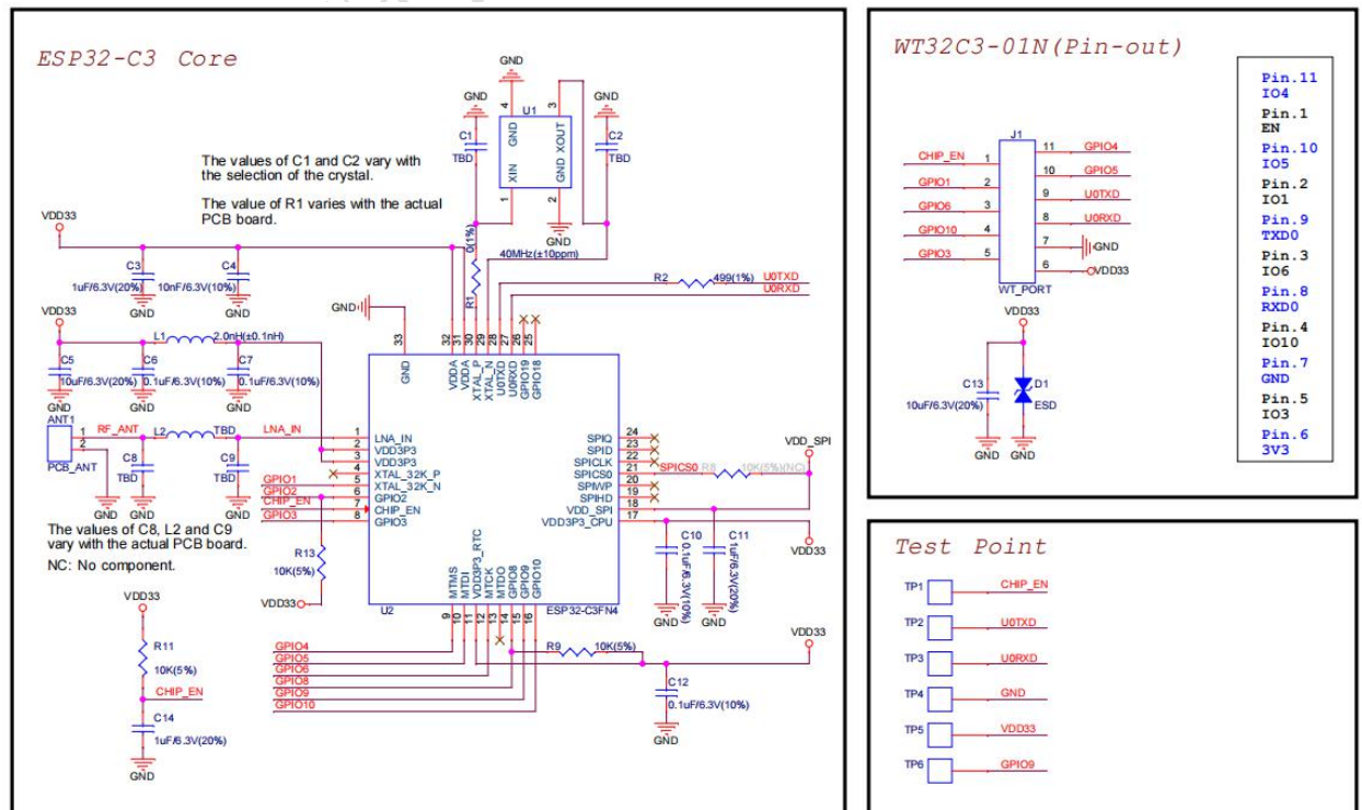
Figure 6 Module Schematics
