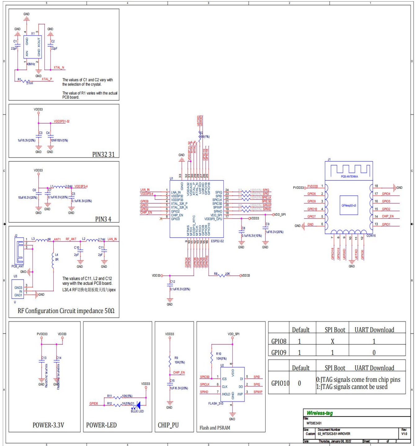
Figure 6 Module Schematics
