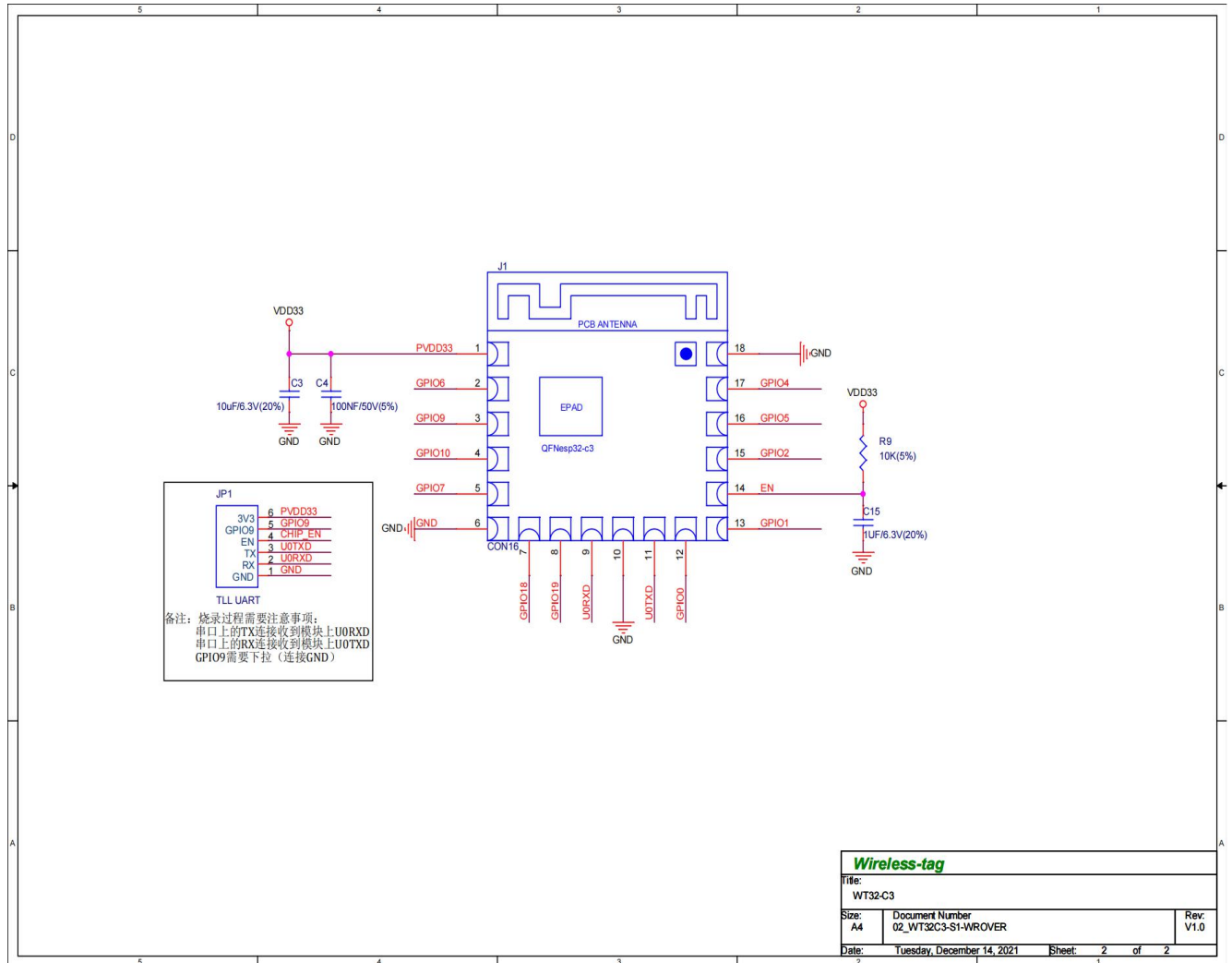
Figure 7 Application Circuit
