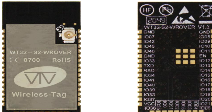
Figure 2 Pin Layout
