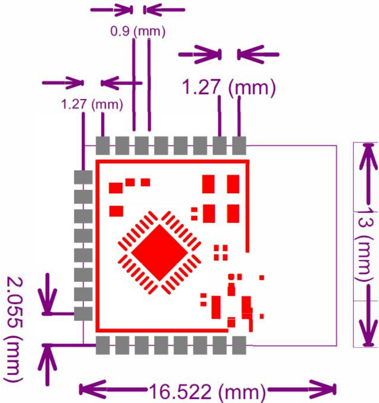
Figure 1 Chip Dimensions
