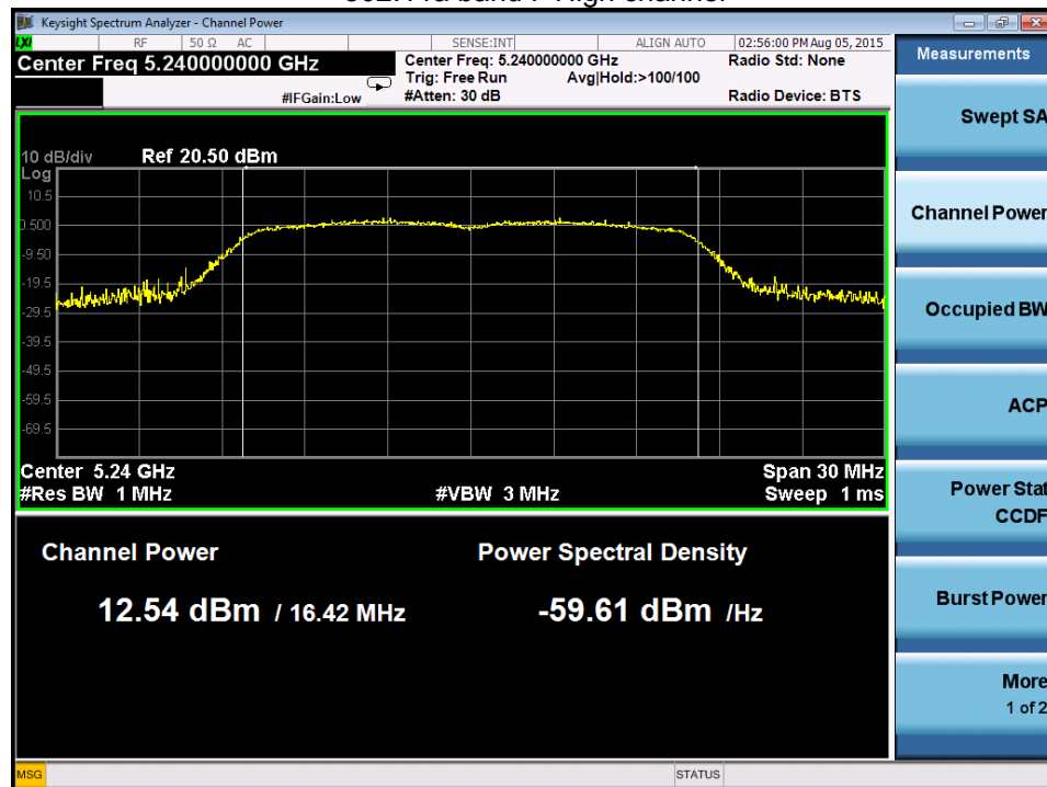
802.11a band I High channel
