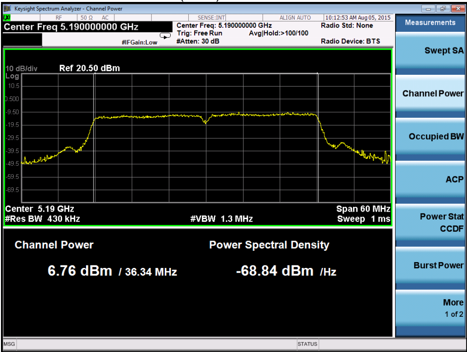
802.11n(HT40) band I Low channel
