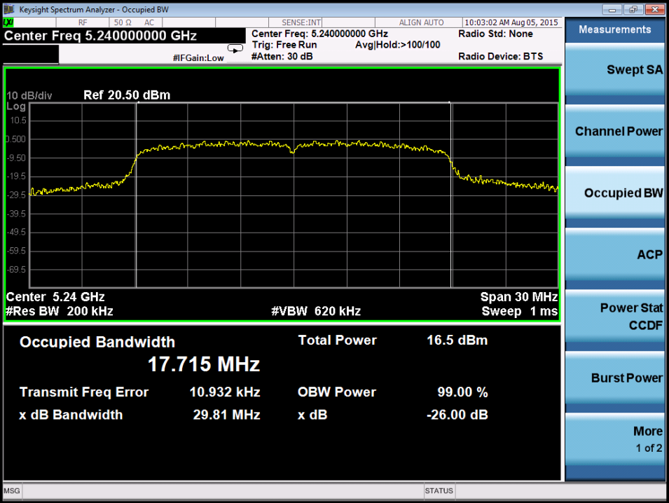
802.11n(HT20) band I High channel
