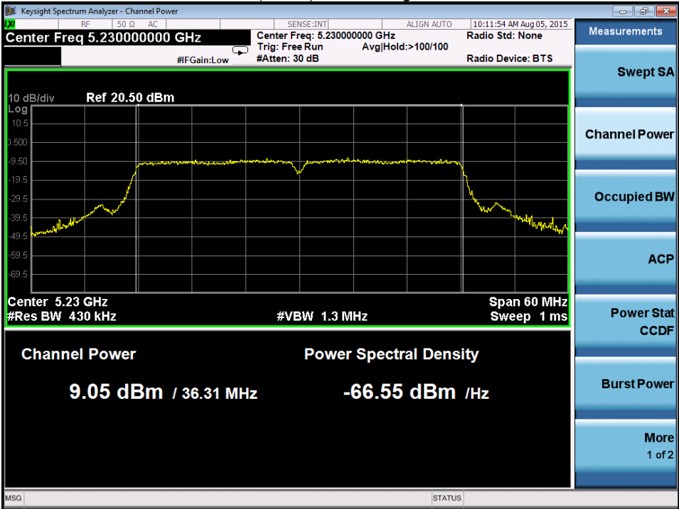
802.11n(HT40) band I High channel
