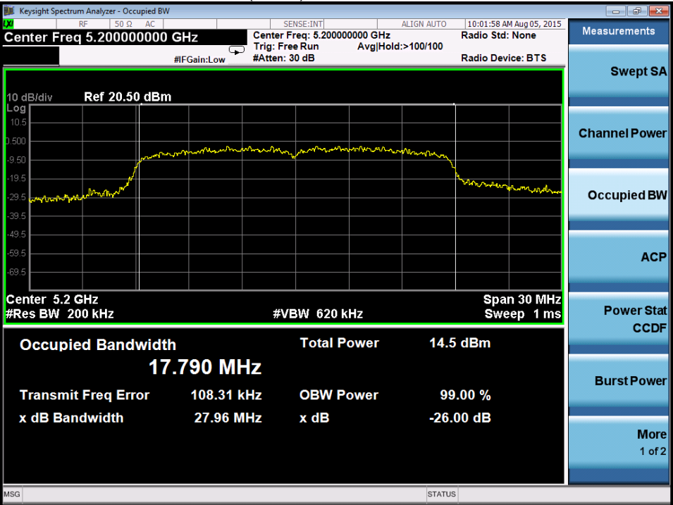
802.11n(HT20) band I Middle channel
