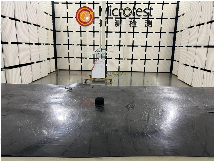
Radiated emissions (below 1GHz) -BT&BLE
