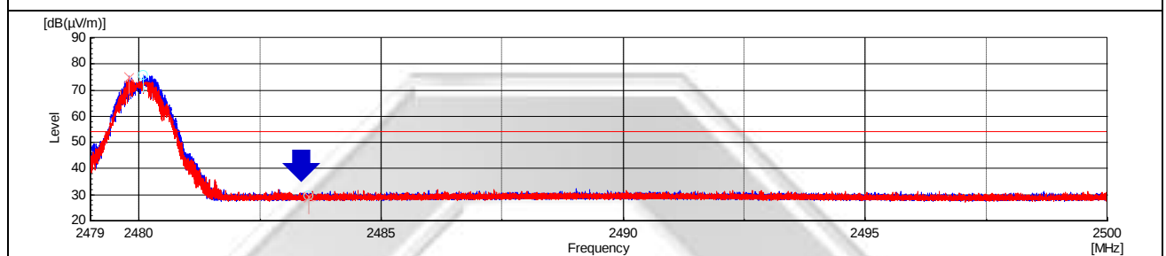
Plot 43 – Upper Band Edge at 2.4835GHz
