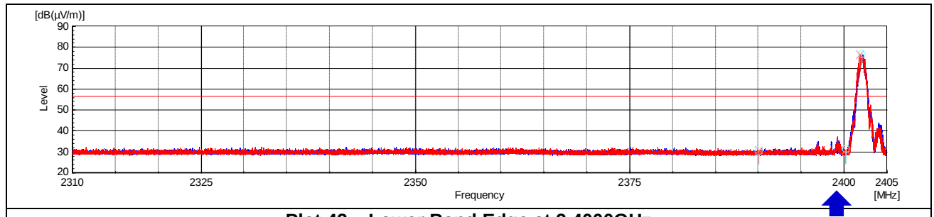
Plot 42 – Lower Band Edge at 2.4000GHz
