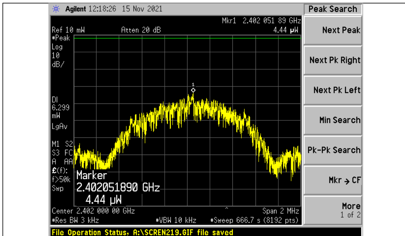
Plot 48 – Lower Channel
