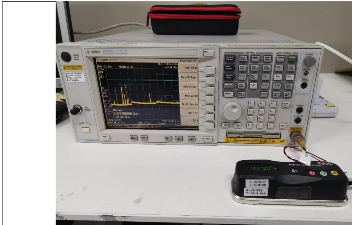
Spectrum Bandwidth (6db Bandwidth Measurement) Test Setup
