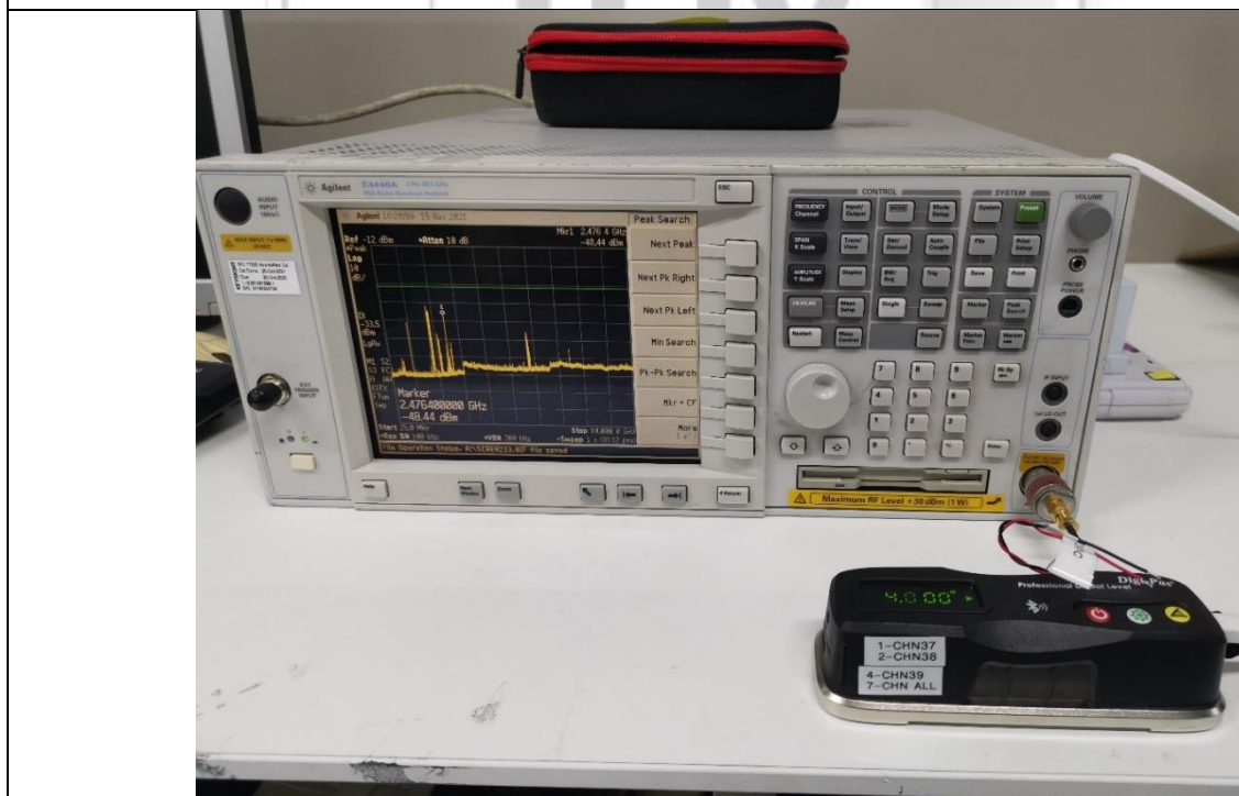
Maximum Peak Power Test Setup
