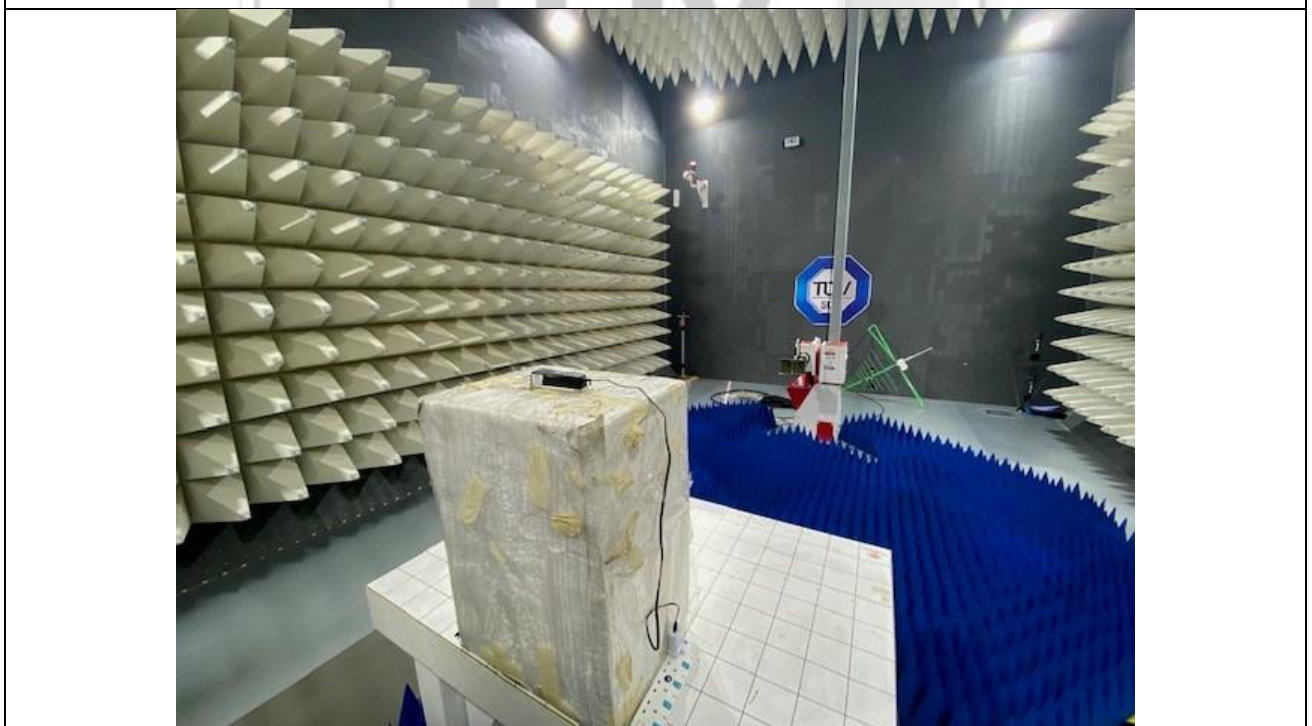
Band Edge Compliance (Radiated) Test Setup
