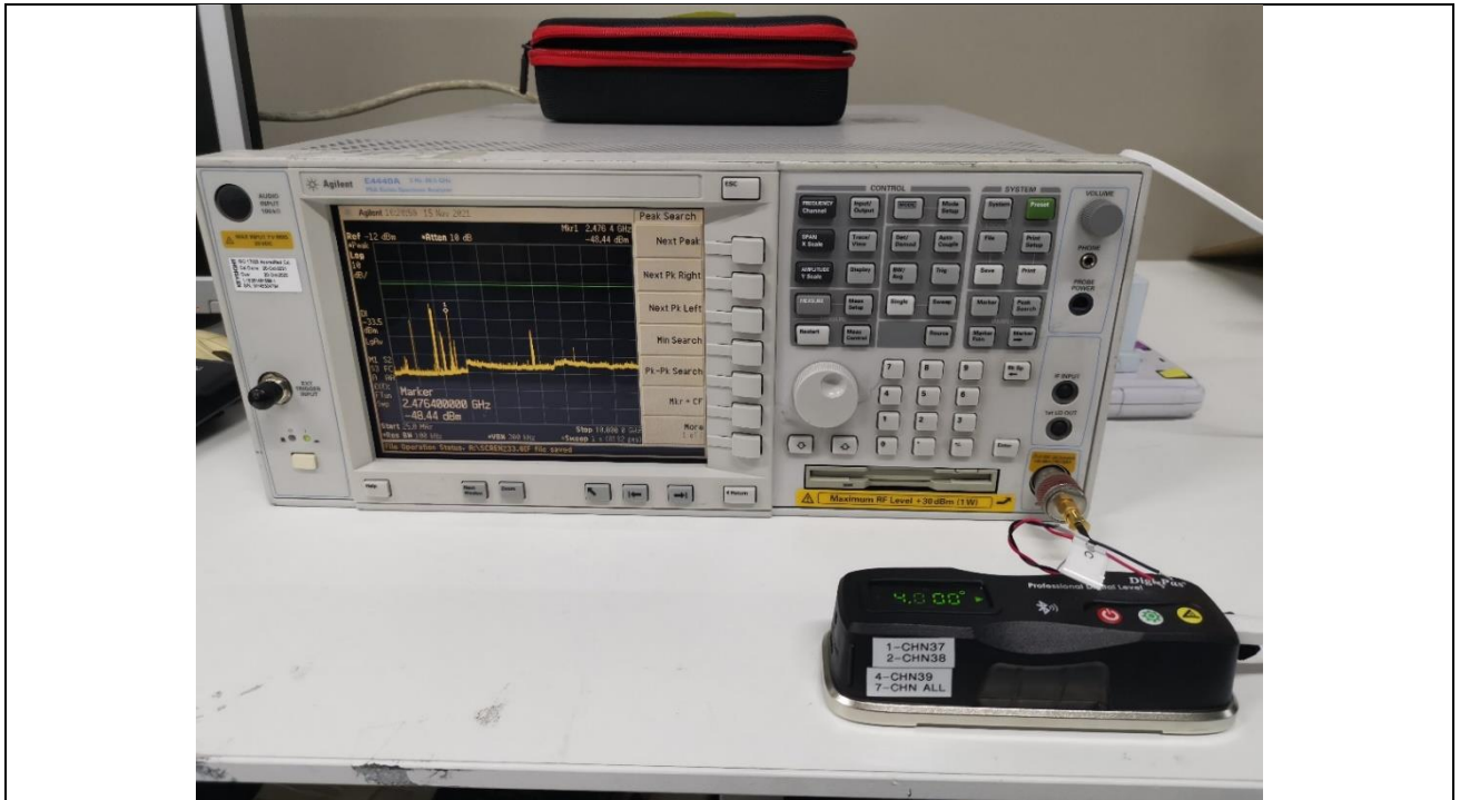
Band Edge Compliance (Conducted) Test Setup
