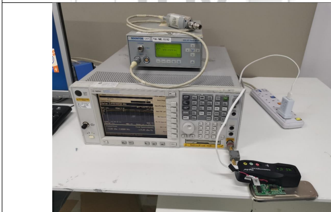
RF Conducted Spurious Emissions (Restricted Bands) Test Setup
