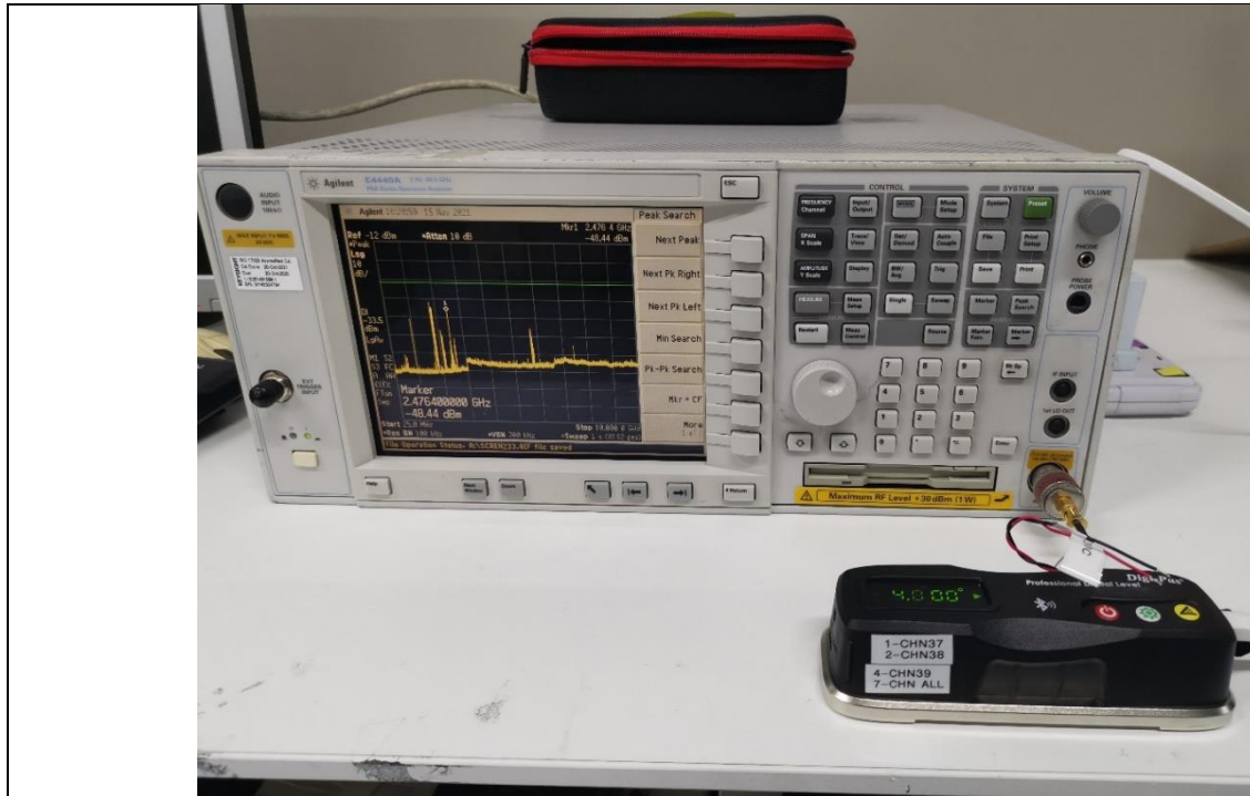
RF Conducted Spurious Emissions (Non-Restricted Bands) Test Setup
