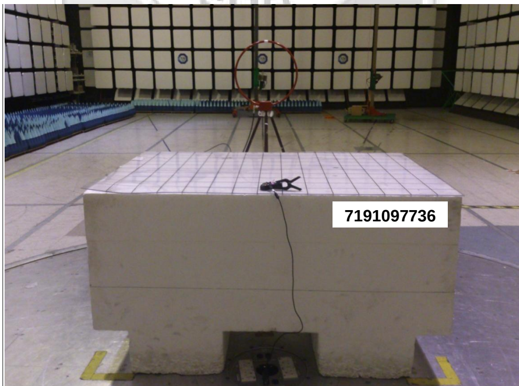
Radiated Emission (Fundamental) Test Setup (Rear View)
