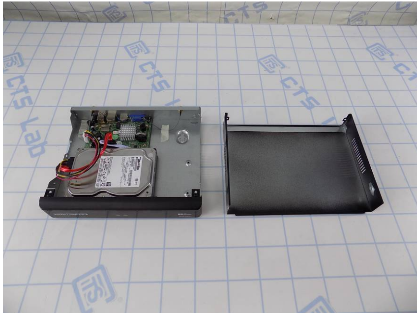
Internal view 1
