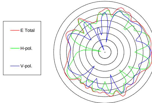
Main antenna @5.6475 GHz
