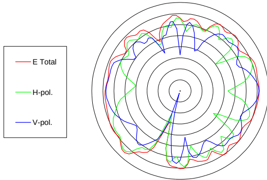
Main antenna @5.15 GHz
