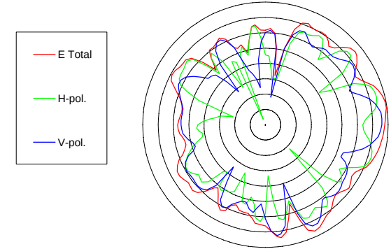
Main antenna @5.825 GHz
