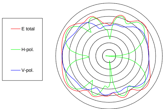
Aux antenna @2.40 GHz
