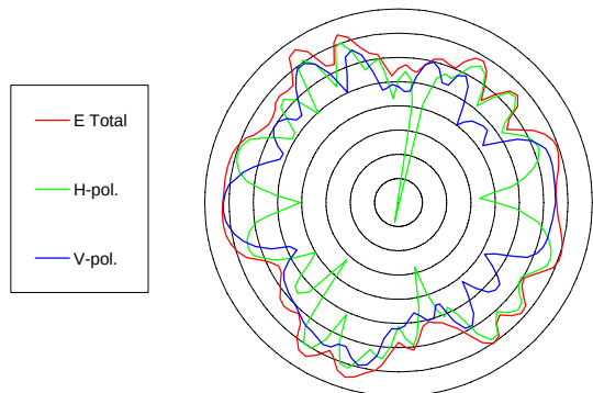
Aux antenna @5.15 GHz
