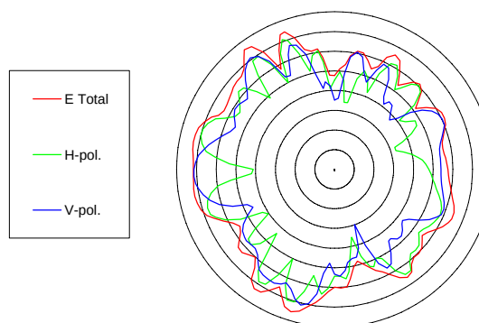
Aux antenna @5.25 GHz
