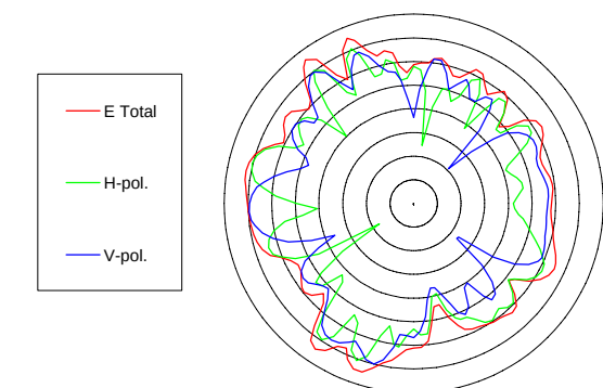
Aux antenna @5.35 GHz
