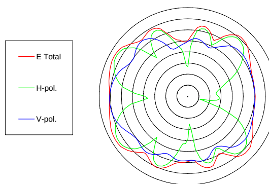
Aux antenna @2.45 GHz
