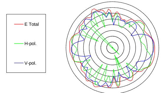
Aux antenna @5.825 GHz
