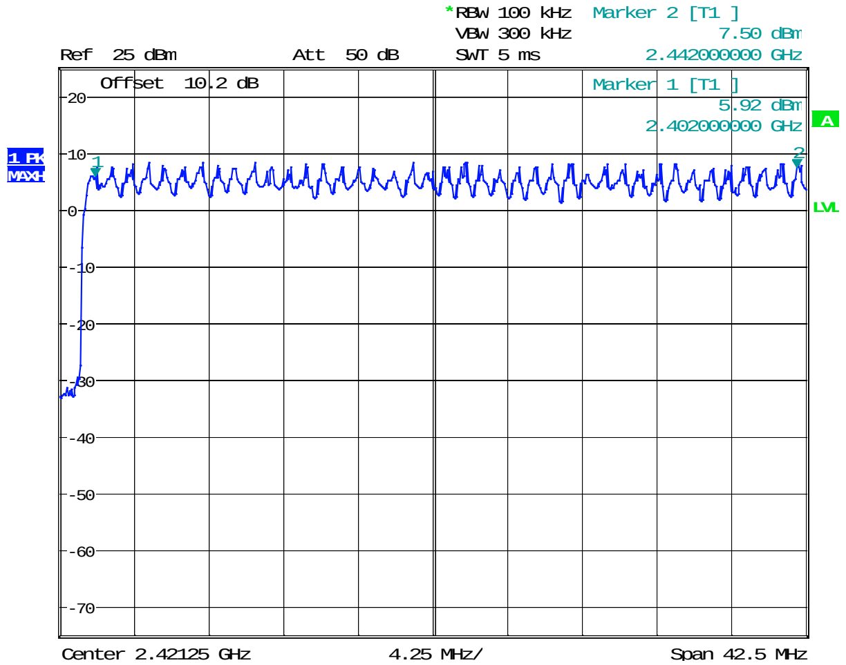
Plot 4.5 - Number of hopping channels (8DPSK - 2400 to 2442.5 MHz)
