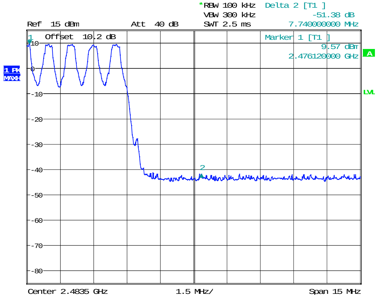
Plot 4.13 Conducted Band Edge, High Channel with GFSK (Hopping)
