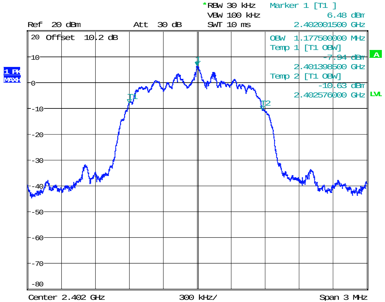
Plot 1. 53 – 99% Bandwidth Low Channel \pi/4 -DQPSK
