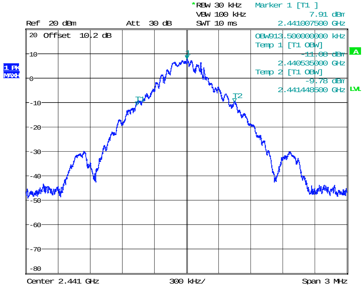
Plot 1. 31- 99% Bandwidth Middle Channel GFSK
