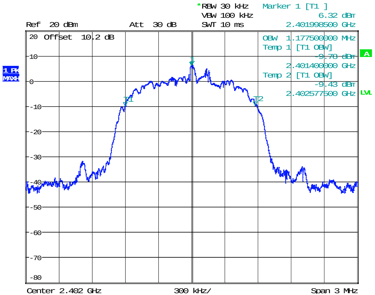
Plot 1. 16 – 99% Bandwidth Low Channel 8DPSK
