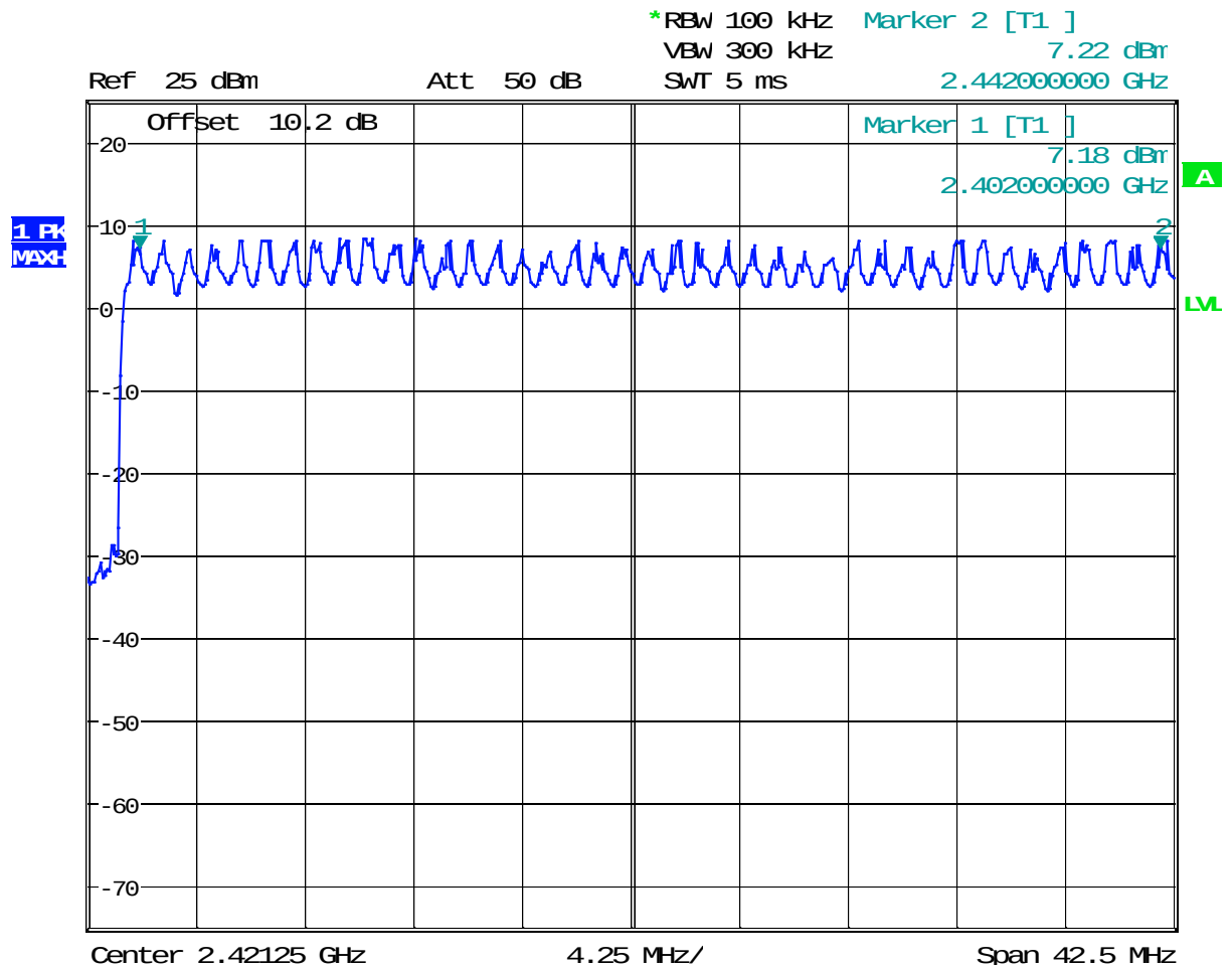
Plot 4.3 - Number of hopping channels ( \pi/4 -DQPSK- 2400 to 2442.5 MHz)
