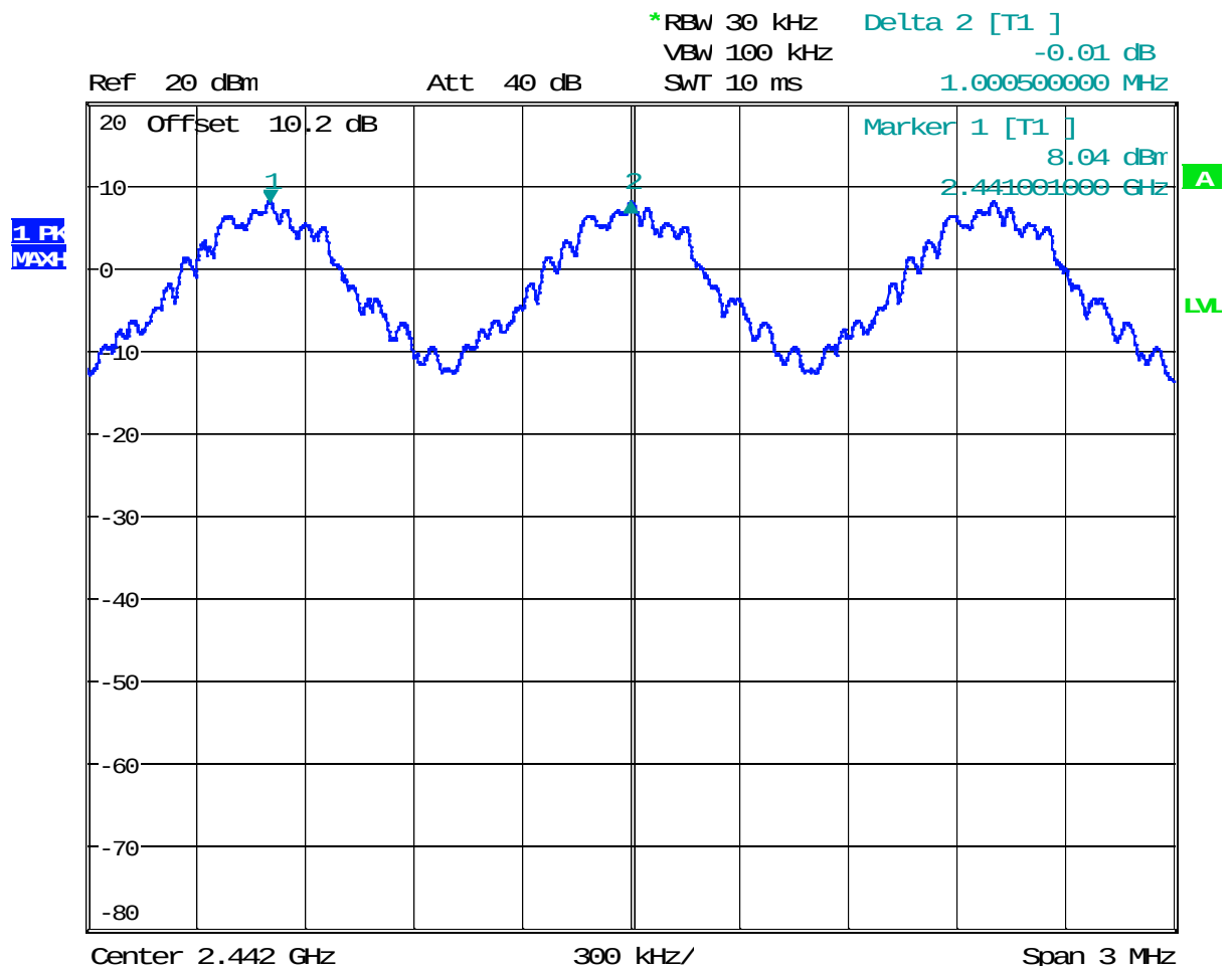
Plot 3.7- Channel Separation GFSK
