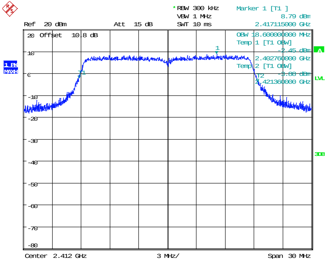
Plot 1.19 – 99% Bandwidth
