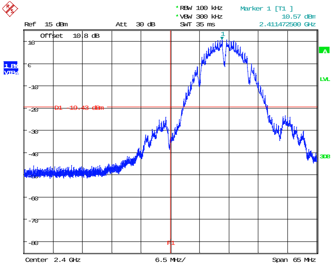
Plot 4.13 Conducted Band Edge, Tx @ 2412MHz 802.11b
