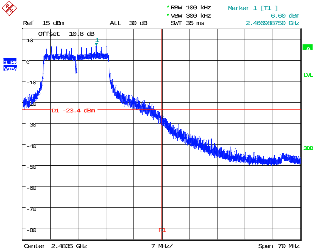
Plot 4.18 Conducted Band Edge, Tx @ 2462MHz 802.11g
