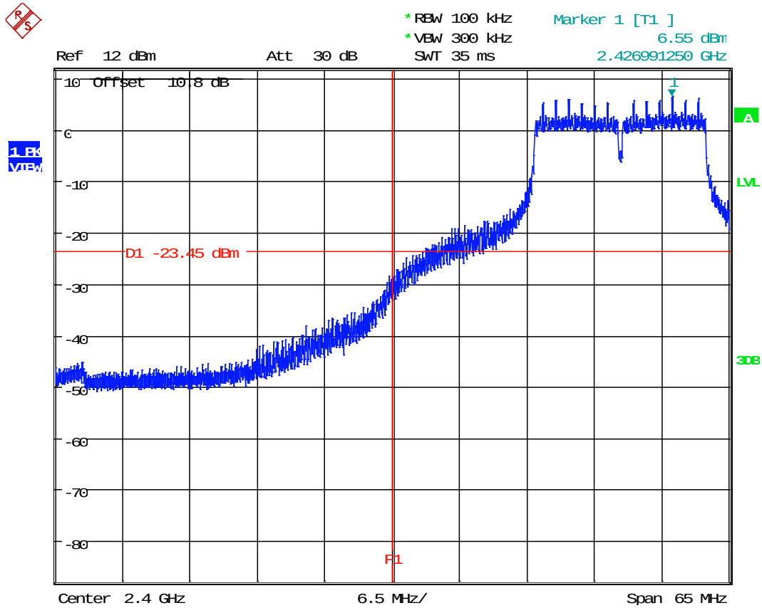
Plot 4.17 Conducted Band Edge, Tx @ 2422MHz 802.11g
