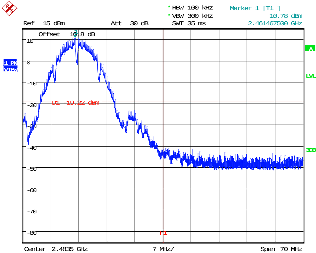
Plot 4.14 Conducted Band Edge, Tx @ 2462MHz 802.11b
