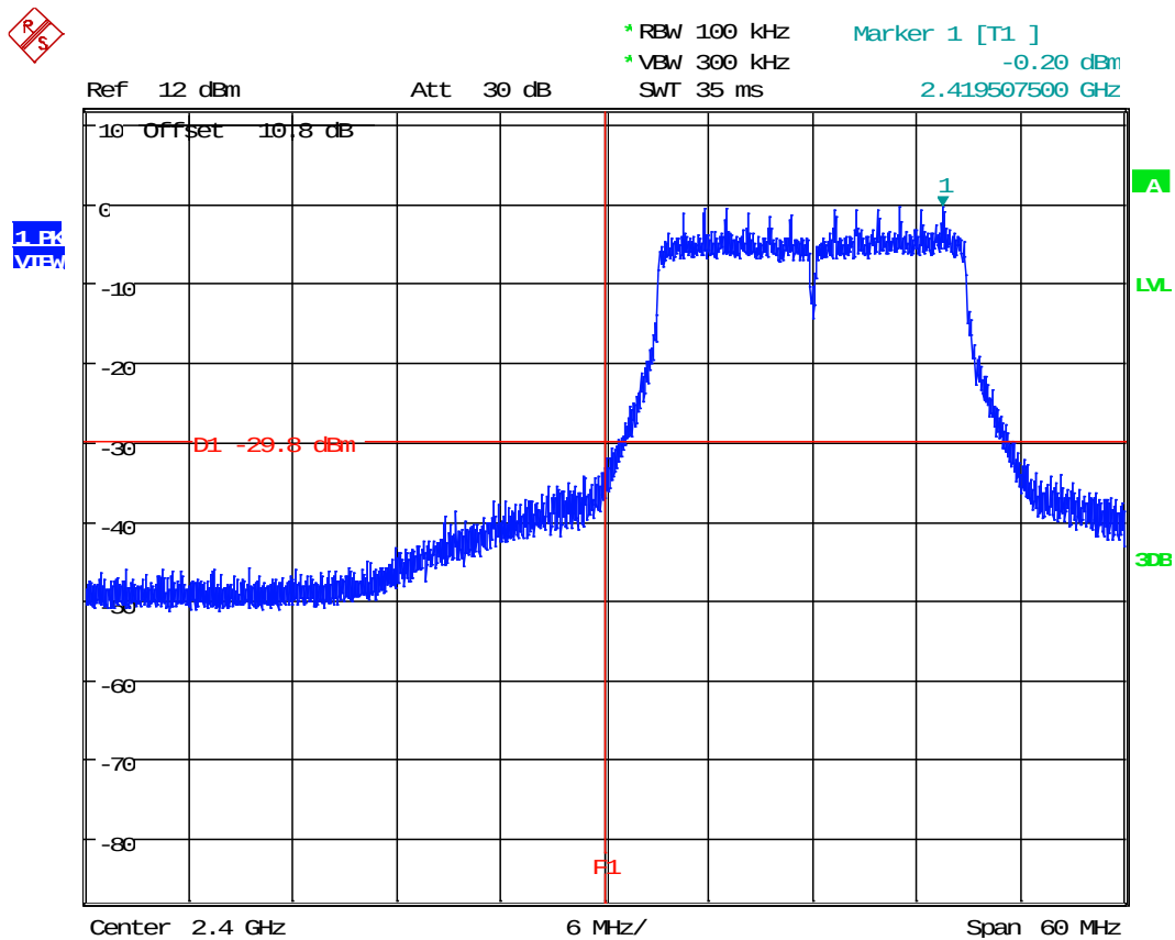
Plot 4.19 Conducted Band Edge, Tx @ 2412MHz 802.11n 20MHz (Power 10.46dBm)
