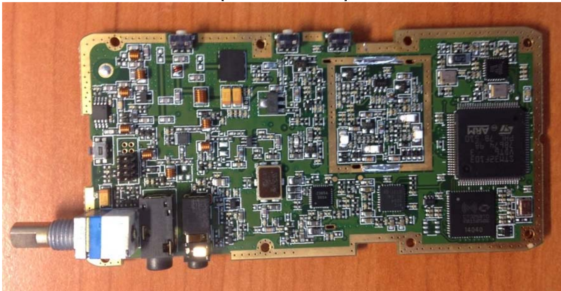
[Main board Rear without shield]
