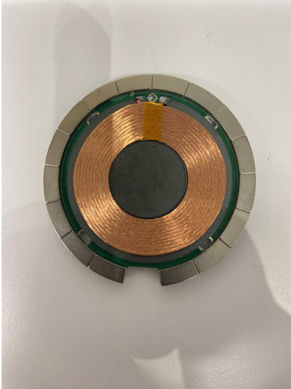
Figure 1: WPT PCB Front
