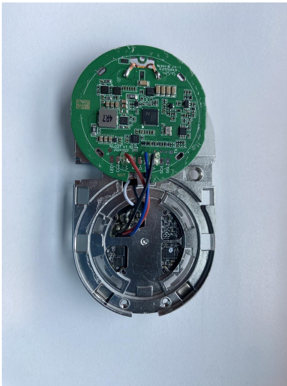
Figure 5: Assembled View
