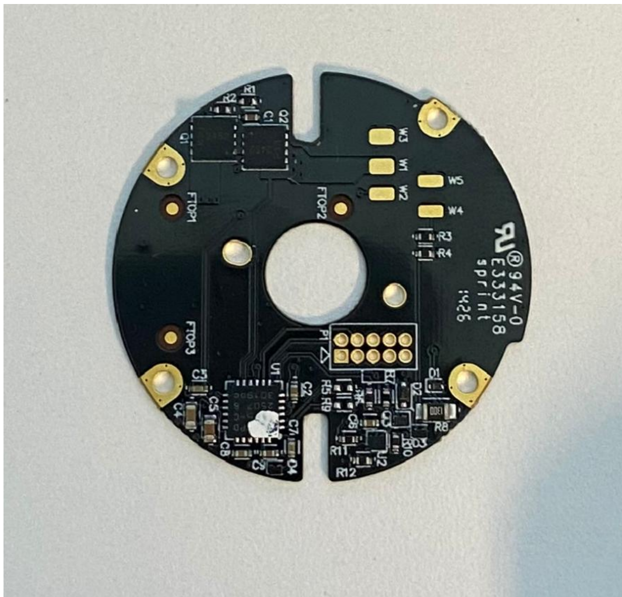
Figure 3: Controller PCB Front
