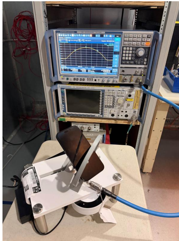
Figure 7: EUT – Conducted Measurements Test Setup
