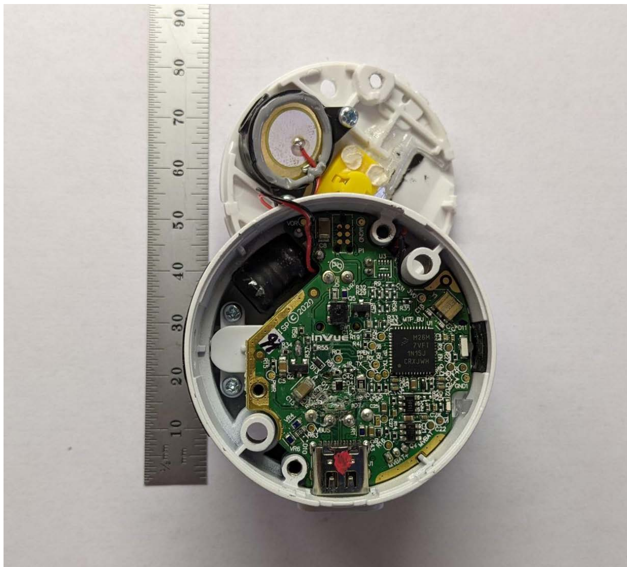
Figure 5: Module Installed in LiveOnePod Host Device
