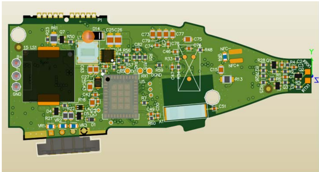
Figure 1: Front View with New Antenna
