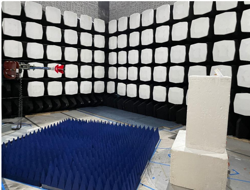
Figure:3 – Test Set up - Radiated Emissions <10 GHz
