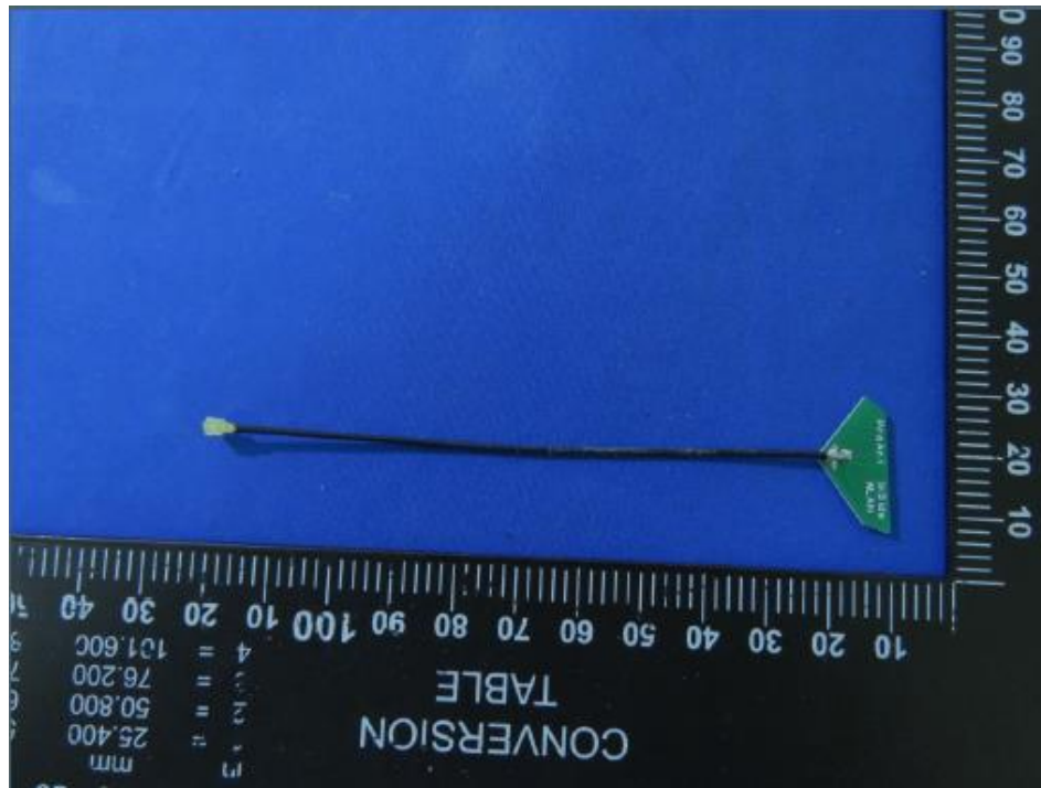
Dipole Antenna (inside WLAN PRO-IS-299)
