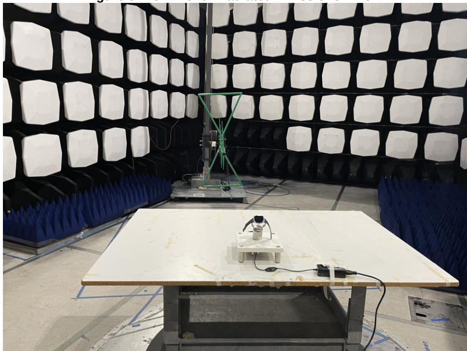
Figure 4: EUT Rear - Radiated Emissions <1 GHz
