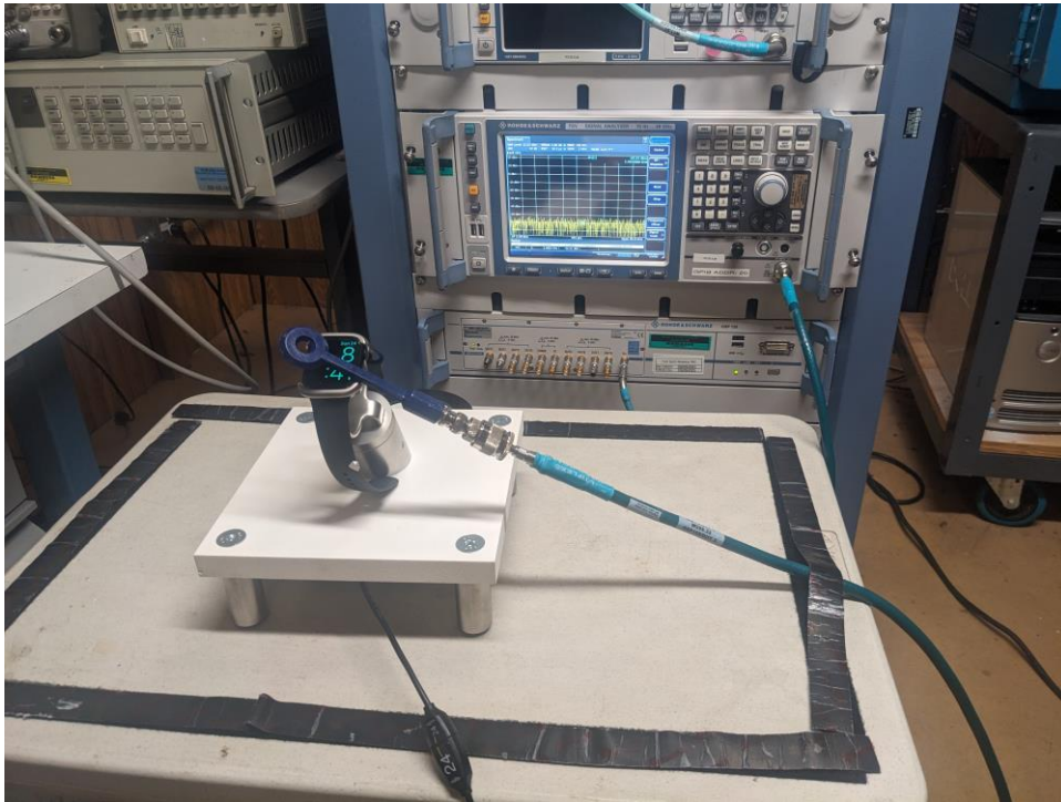
Figure 7: EUT – Conducted Measurements Test Setup
