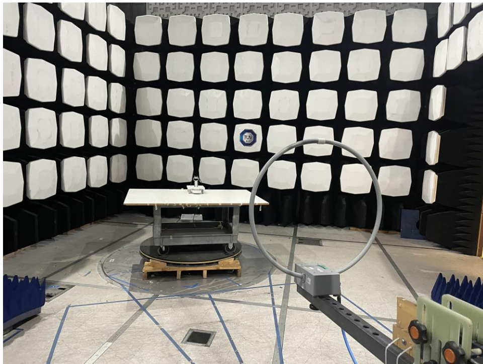
Figure 1: EUT Front - Radiated Emissions < 30 MHz
