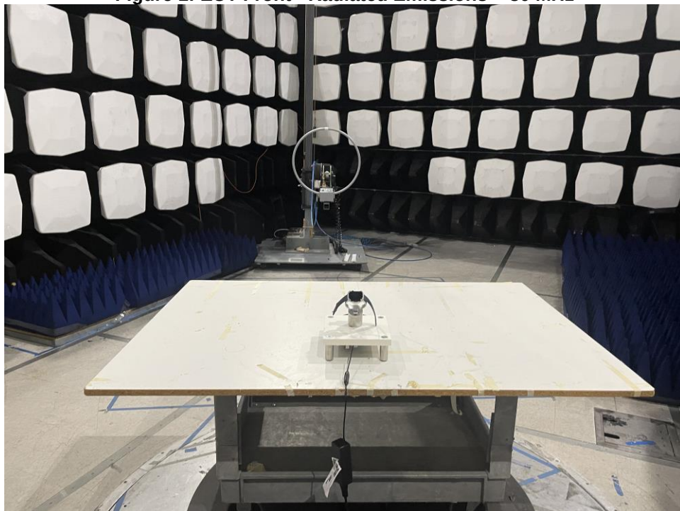
Figure 2: EUT Rear - Radiated Emissions < 30 MHz
