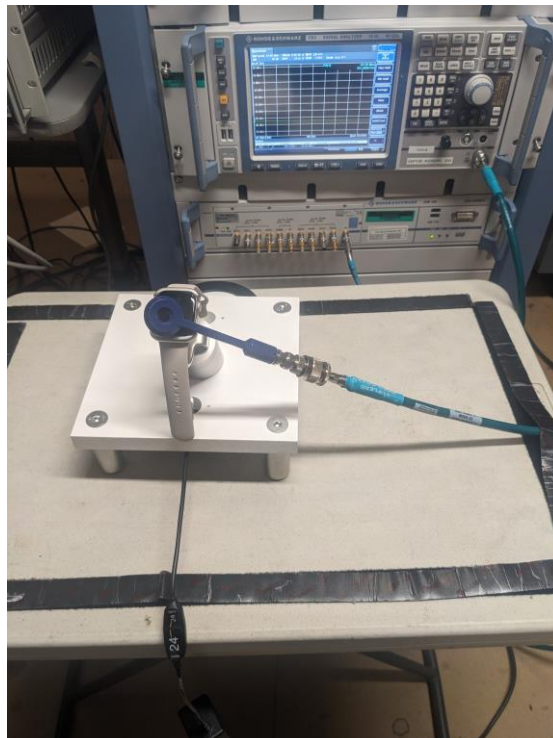
Figure 8: EUT – Conducted Measurements Test Setup
