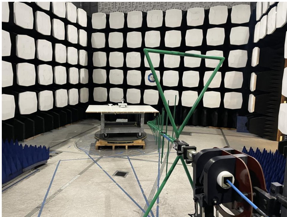
Figure 3: EUT Front - Radiated Emissions <1 GHz
