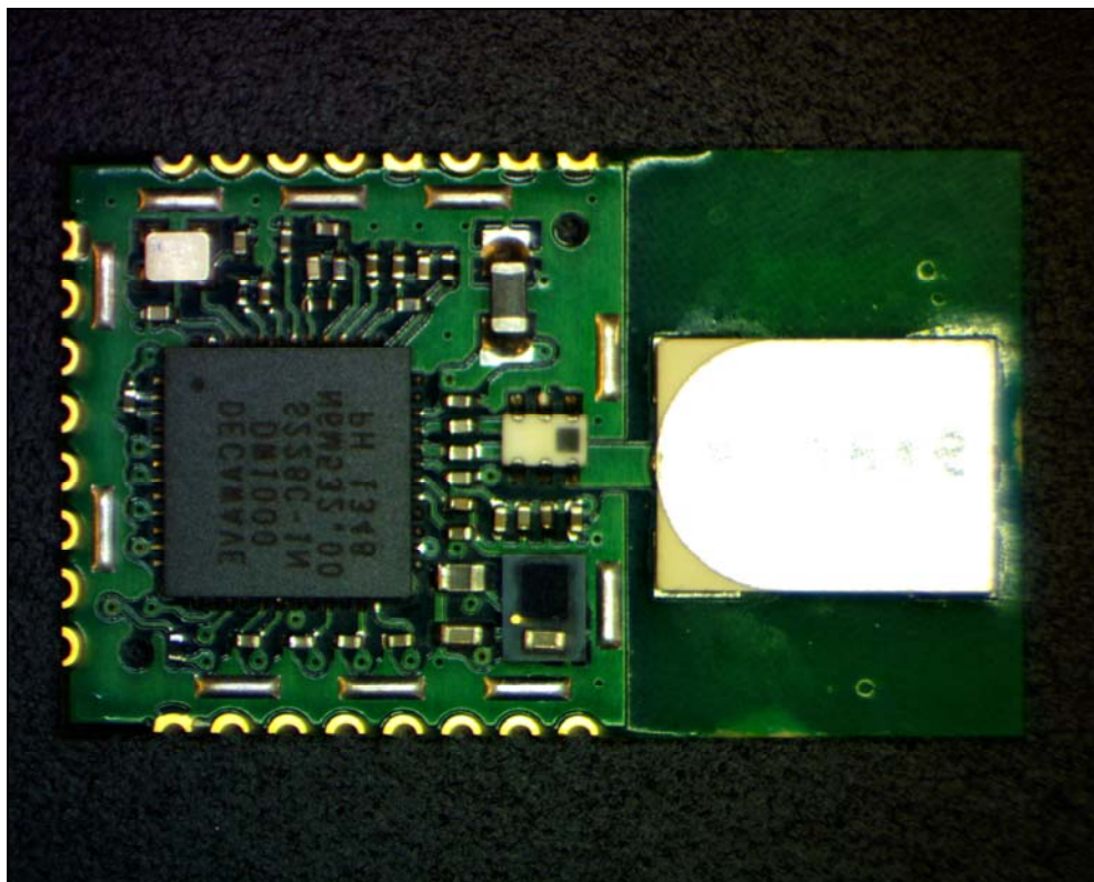
Figure 2: PCB without Shield - Front
