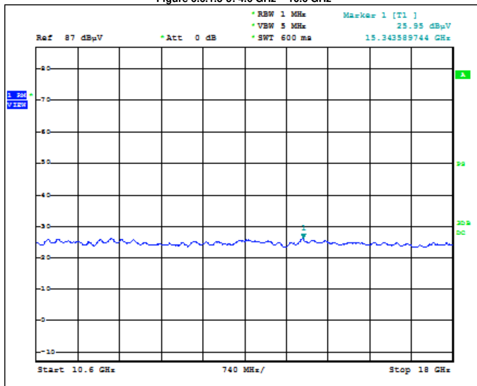
Figure 6.6.1.3-6: 10.6 GHz – 18 GHz
