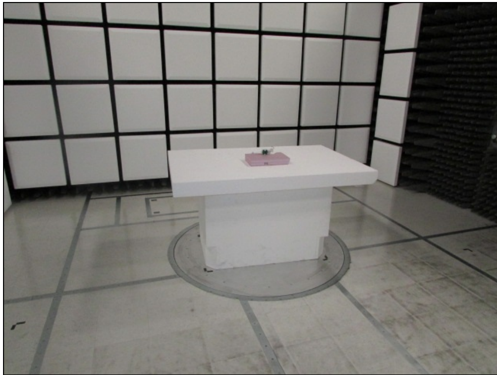
Figure 5: Radiated Emissions – Below 1GHz
