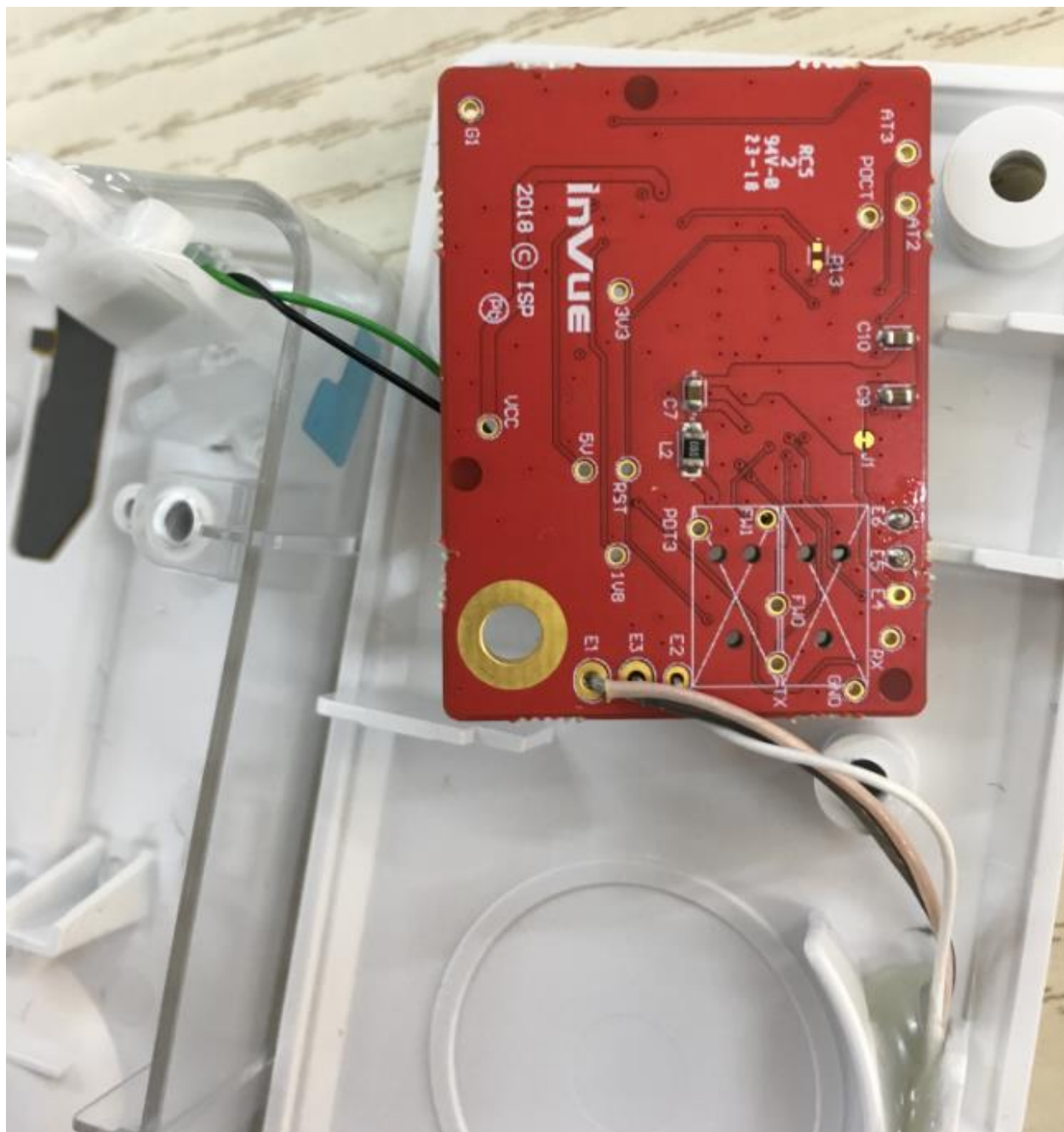
PCBA Bottom View Taken out from Plastic
