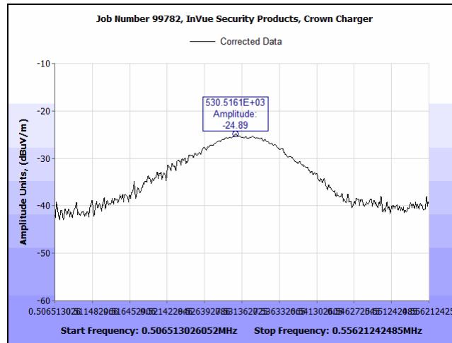
Plot 9. Radiated Emission – Fundamental, Vertical Unit, Plot
