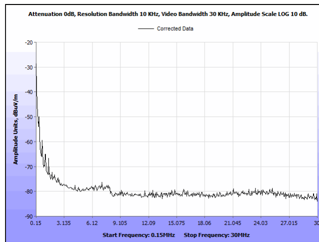
Plot 12. Radiated Emission – (150kHz – 30MHz), Horizontal Unit, Plot
