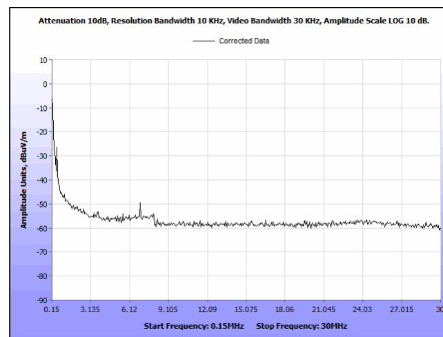
Plot 7. Radiated Emission – (150 kHz – 30 MHz), Vertical Unit, Pen Charging Plot
