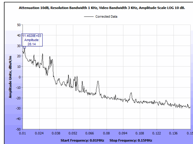
Plot 6. Radiated Emission – (10 – 150 kHz), Vertical Unit, Pen not Charging Plot
