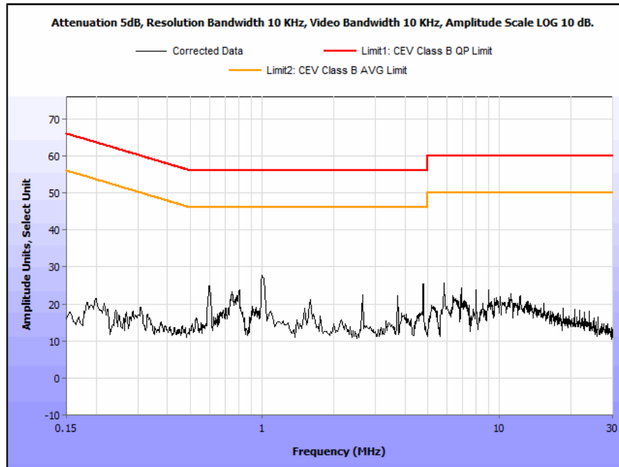
Plot 3. Conducted Emissions at the Mains Terminal Test Data, Horizontal Unit – Phase Plot
