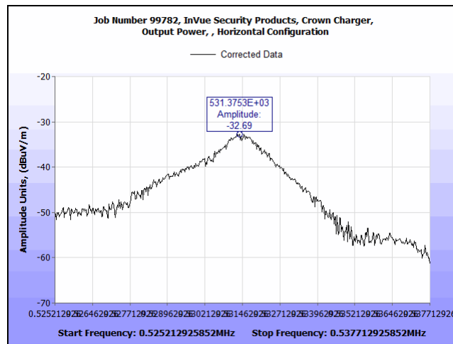
Plot 10. Radiated Emission – Fundamental, Horizontal Unit, Plot
