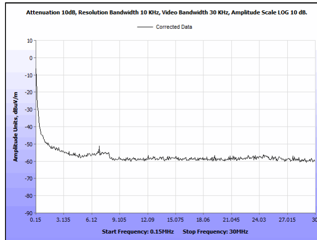
Plot 8. Radiated Emission – (150 kHz – 30 MHz), Vertical Unit, Pen not Charging Plot
