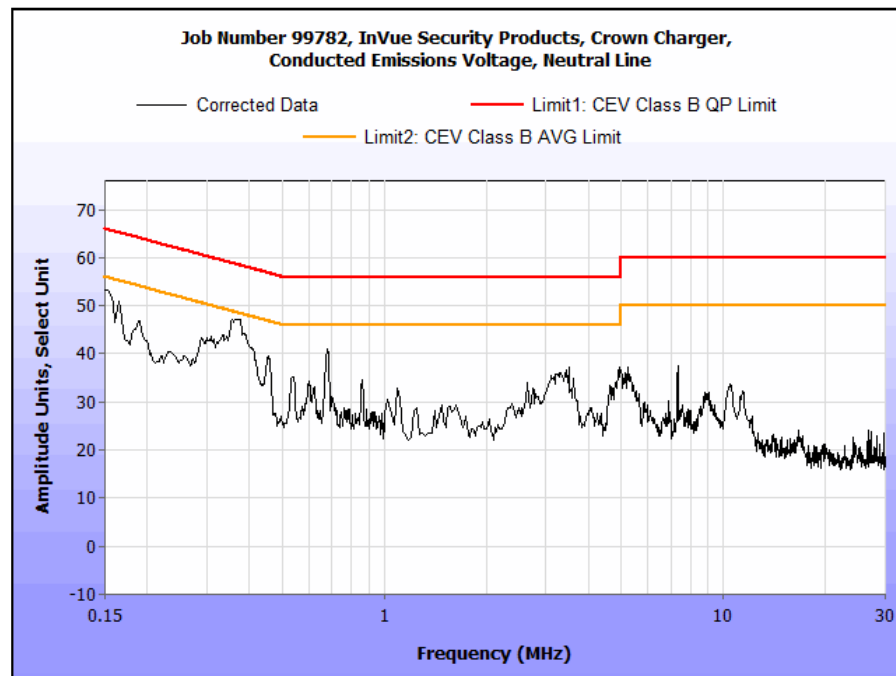
Plot 2. Conducted Emissions at the Mains Terminal Test Data, Vertical Unit – Neutral Plot
