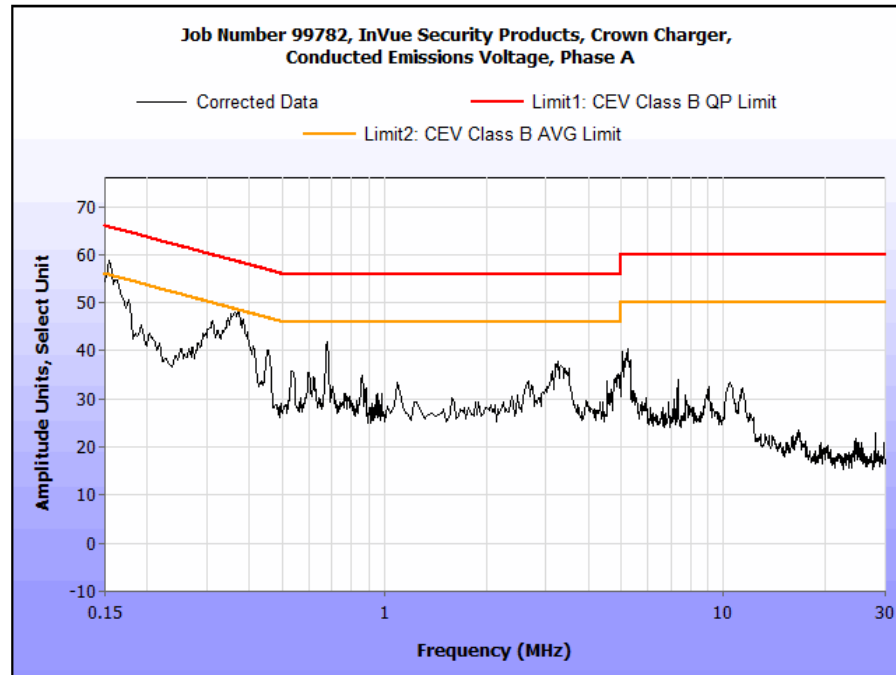
Plot 1. Conducted Emissions at the Mains Terminal Test Data, Vertical Unit – Phase Plot
