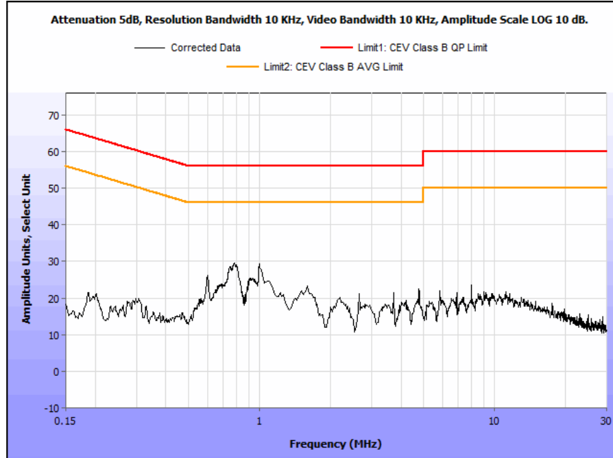
Plot 4. Conducted Emissions at the Mains Terminal Test Data, Horizontal Unit – Neutral Plot
