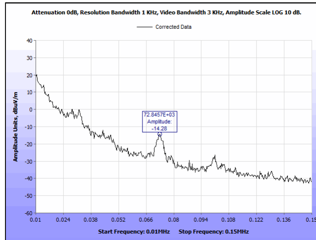
Plot 11. Radiated Emission – (10 - 150 kHz), Horizontal Unit, Plot
