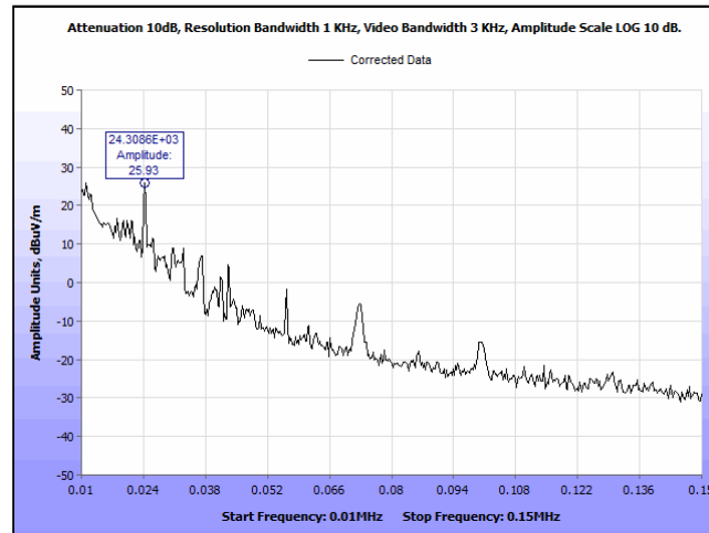
Plot 5. Radiated Emission – (10 – 150 kHz), Vertical Unit, Pen Charging Plot
