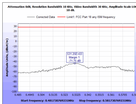
Plots 9. Radiated Emission – Field strength of Operational Band 531 KHz – 562 KHz
