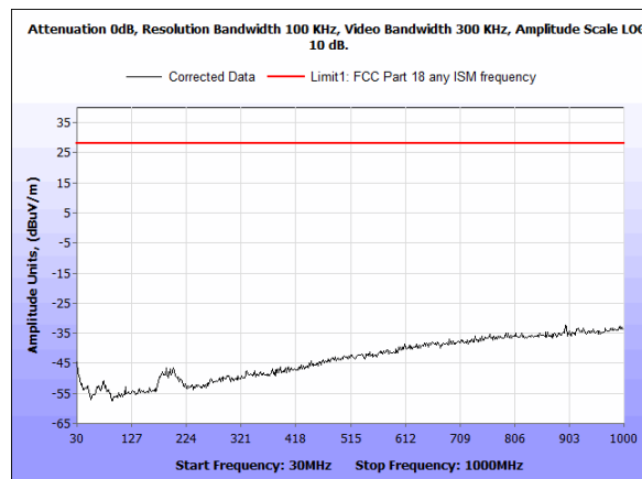
Plots 8. Radiated Emission – (30 MHz - 1 GHz) Vertical
