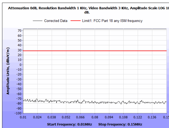
Plots 3. Radiated Emission – (10 kHz – 150 kHz) 0 degree
