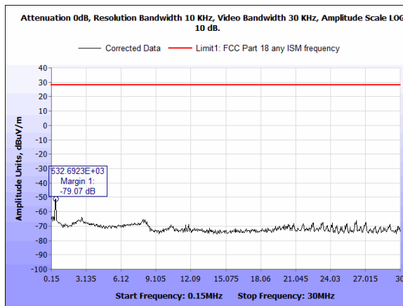
Plots 5. Radiated Emission – (150 kHz – 30 MHz) 0 degree
