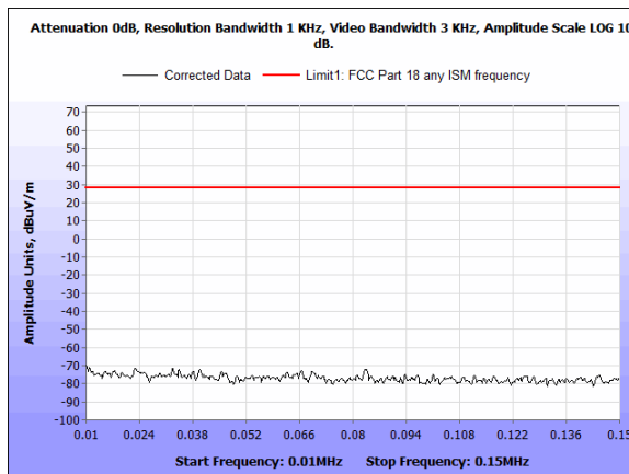
Plots 4. Radiated Emission – (10 kHz – 150 kHz) 90 degree
