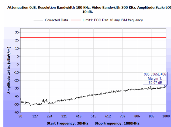
Plots 7. Radiated Emission – (30 MHz - 1 GHz) Horizontal
