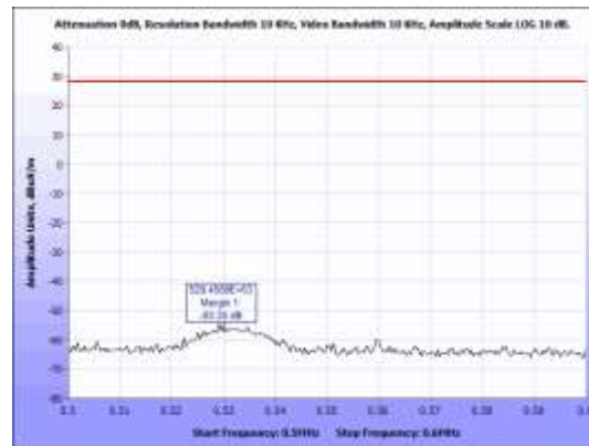
Figure 9: Field Strength Limits, Fundamental Emission, Cumulative
