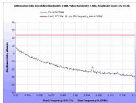
Figure 11: Field Strength Limits, V Unit, 0.01 - 0.15 MHz, Parallel
