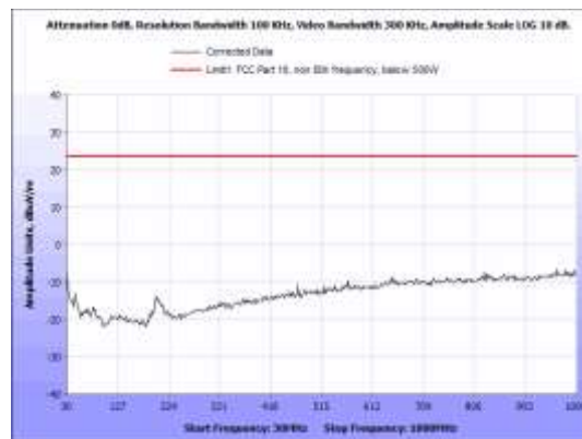
Figure 14: Field Strength Limits, V Unit, 30 - 1000 MHz
