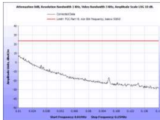
Figure 10: Field Strength Limits, V Unit, 0.01 - 0.15 MHz, Perpendicular
