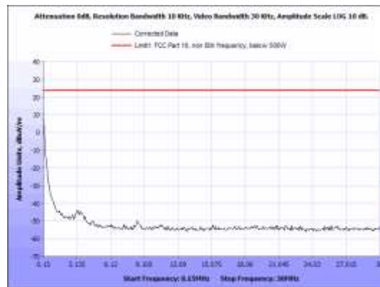
Figure 12: Field Strength Limits, V Unit, 0.15 - 30 MHz, Perpendicular
