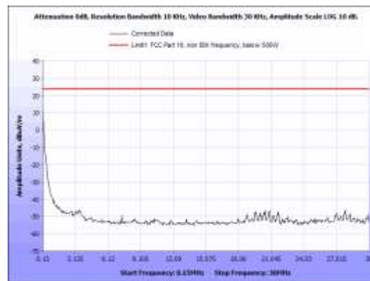
Figure 13: Field Strength Limits, V Unit, 0.15 - 30 MHz, Parallel
