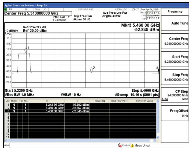
Channel 48 / 5240 MHz – Average IEEE 802.11n HT40
