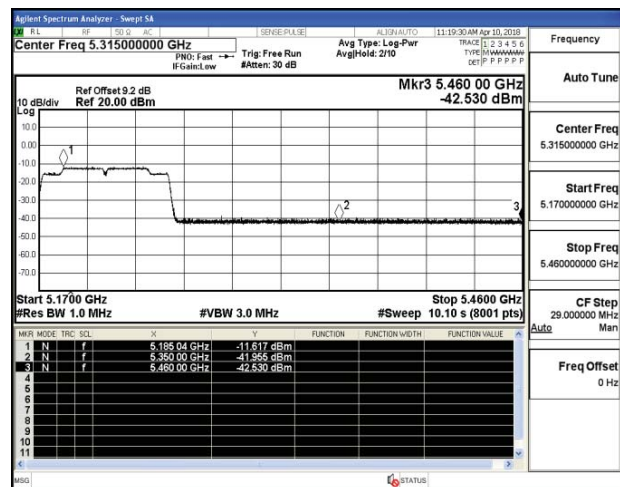
Channel 46 / 5230 MHz – Peak(right)
