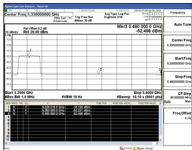
Channel 46 / 5230 MHz – Average
