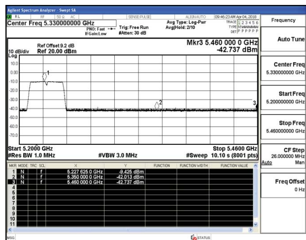
Channel 46 / 5230 MHz – Peak
