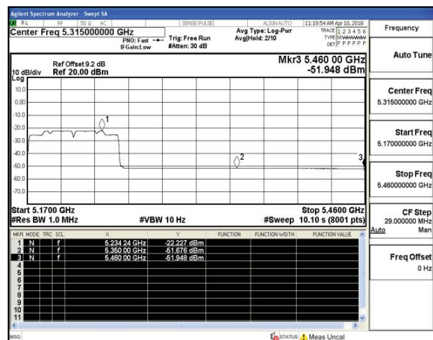
Channel 46 / 5230 MHz – Average(right)
