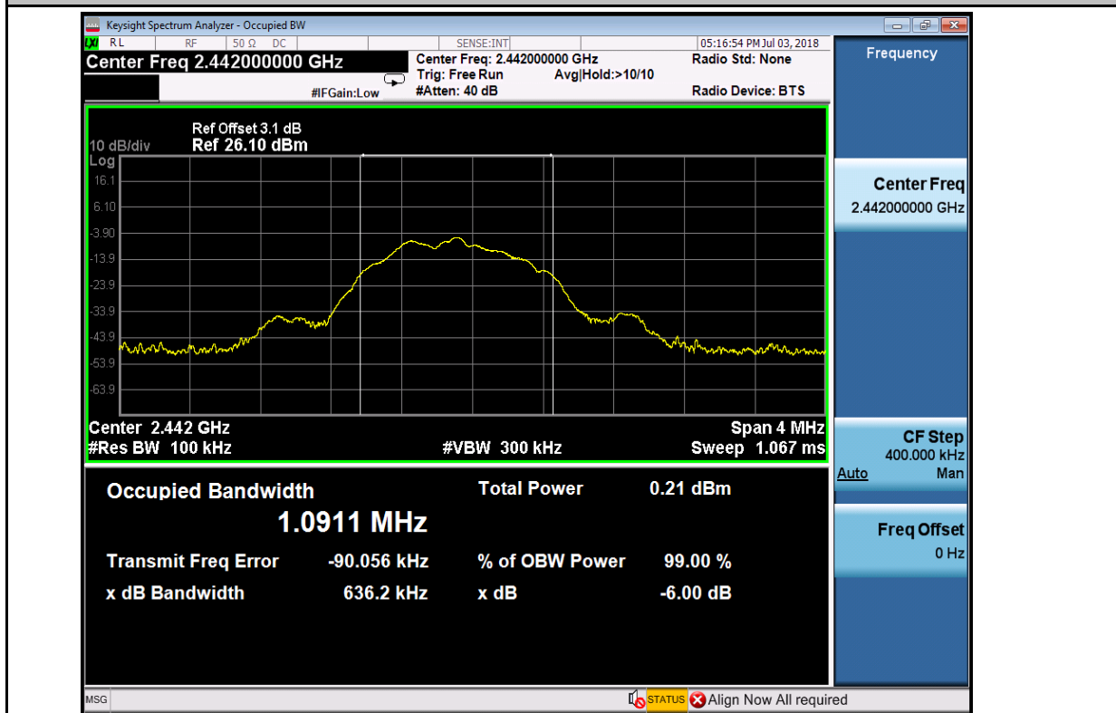
6dB Bandwidth_BLE_2442_Ant1
