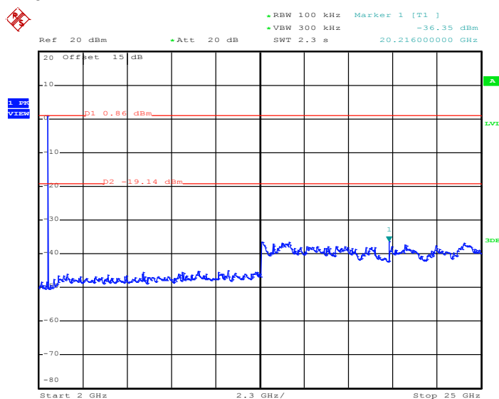
3Mbps CSE Plot on Ch 78 between 2 GHz ~ 25 GHz
