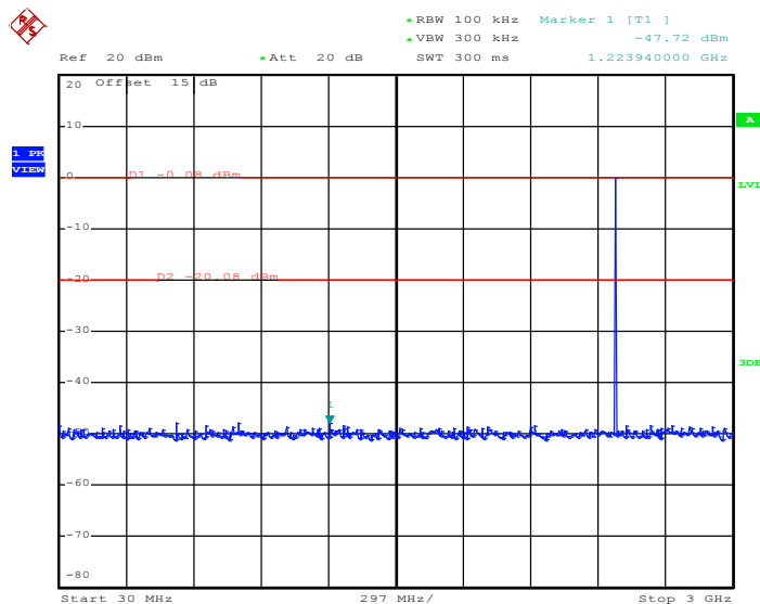
3Mbps CSE Plot on Ch 78 between 30MHz ~ 3 GHz
