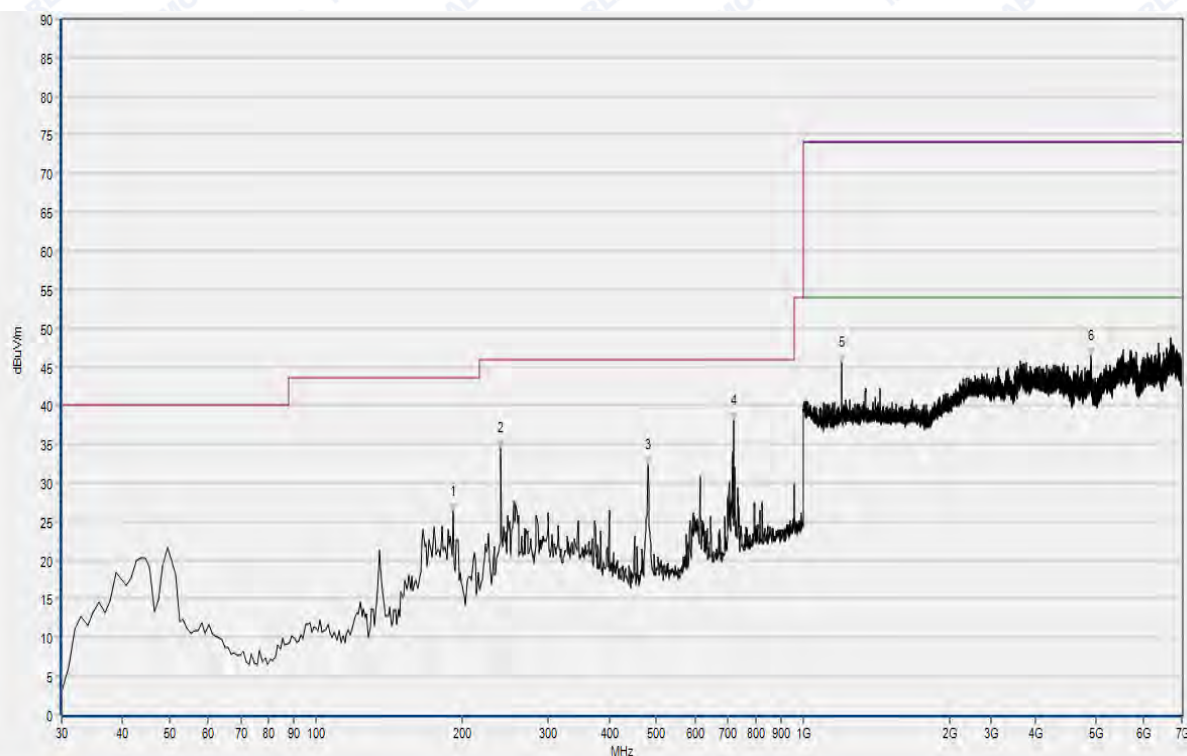
(Plot B: 30MHz – 7GHz, Test Antenna Horizontal)
