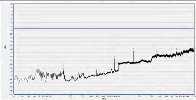
(Plot I3: HSUPA 850MHz Channel = 4175, Test Antenna Horizontal)
