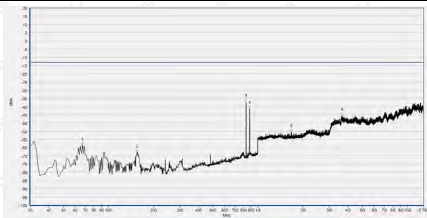
(Plot E3: WCDMA 850MHz Channel = 4175, Test Antenna Horizontal)
