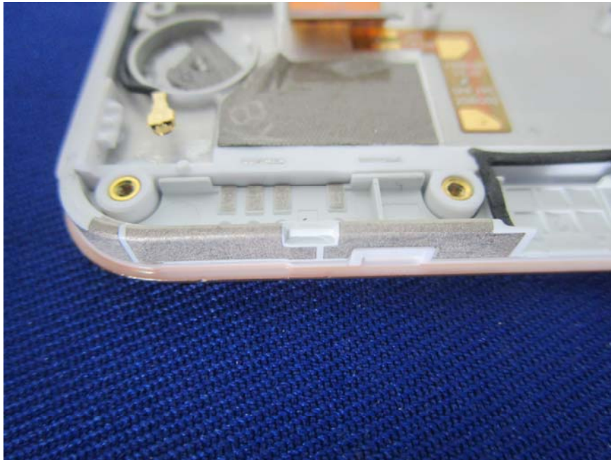
EUT – LTE Main Antenna View
