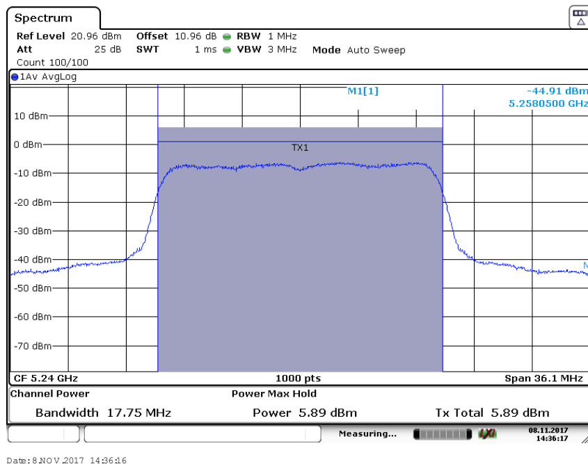
Test Graph 15: 6 Mbps Channel 48 / 5240 MHz path B power
