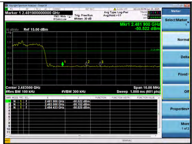
Bluetooth 2DH5
