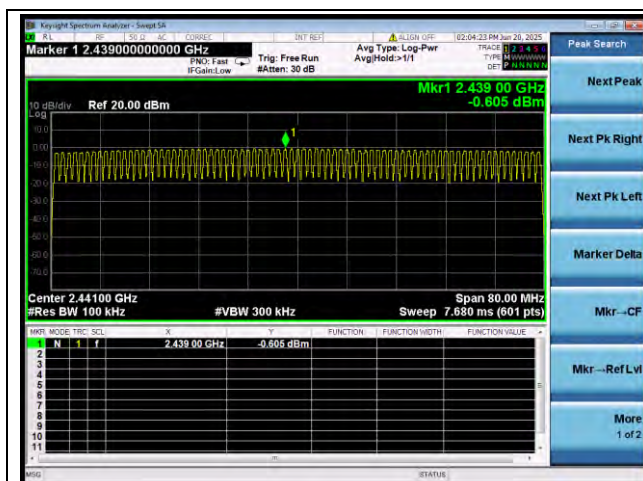
Bluetooth DH5
