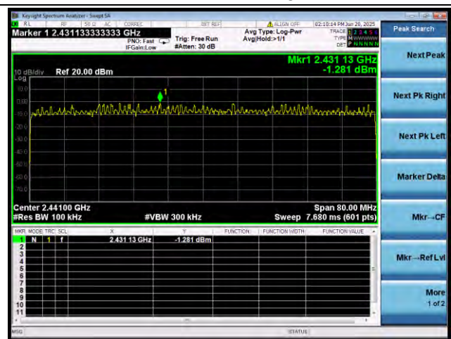
Bluetooth 2DH5
