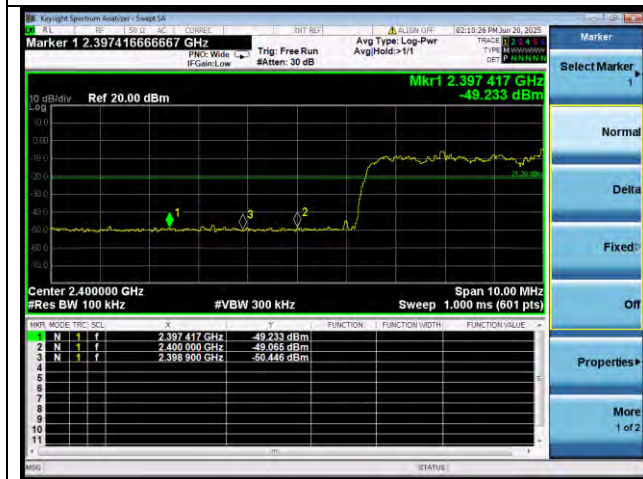
Bluetooth 2DH5
