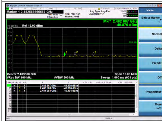
Bluetooth DH5
