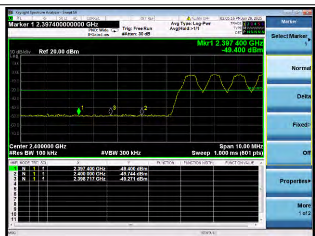
Bluetooth DH5
