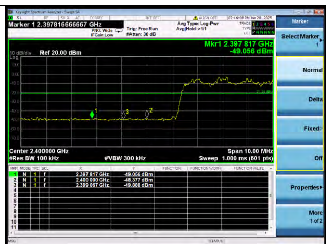
Bluetooth 3DH5
