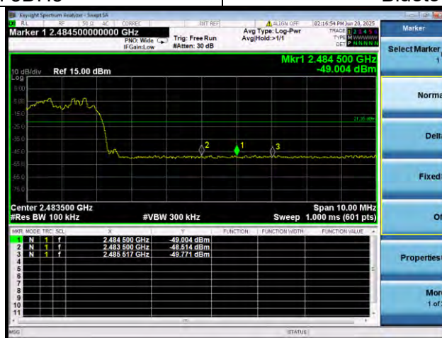
Bluetooth 3DH5
