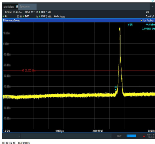
Band7-15MHz-QPSK-21100-75RB#0-1000~300
