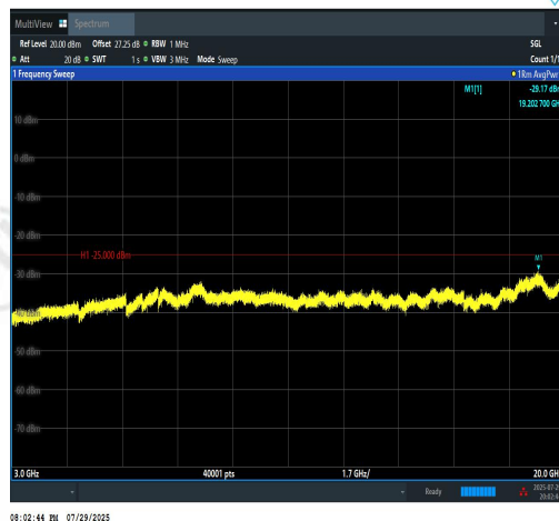
Band7-15MHz-QPSK-21100-75RB#0-3000~200
