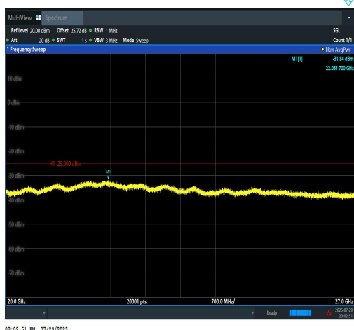
Band7-15MHz-QPSK-21100-75RB#0-20000~27
