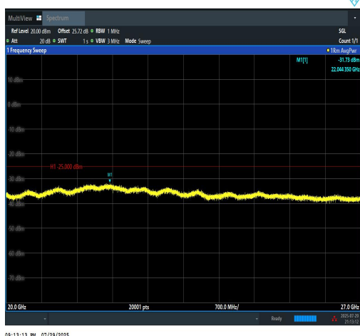
Band7-15MHz-QPSK-21375-1RB#0-20000~270-00-PASS
