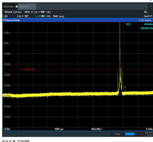
Band7-15MHz-QPSK-21375-1RB#0-1000~3000-PASS
