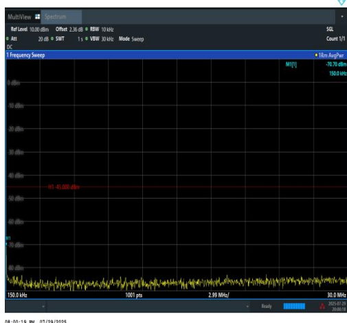
Band7-15MHz-16QAM-21100-1RB#0-0.15~30-P
