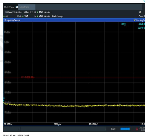
Band7-15MHz-16QAM-21375-75RB#0-30~1000-
