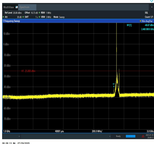
Band7-20MHz-QPSK-20850-1RB#0-1000~3000-
