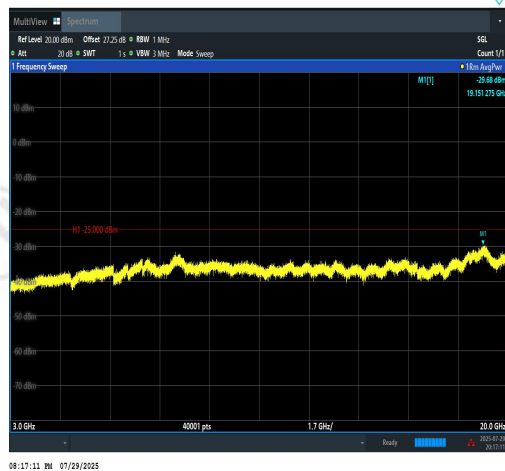
Band7-20MHz-QPSK-20850-100RB#0-3000~20 000-PASS
