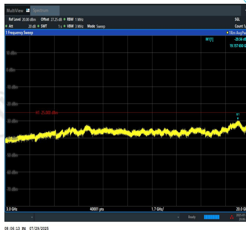
Band7-15MHz-16QAM-21375-1RB#74-3000~20 000-PASS
