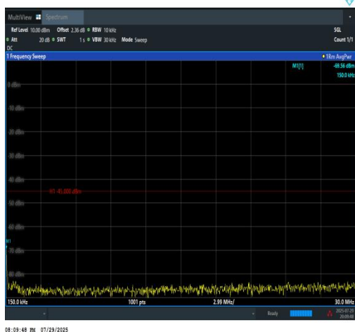
Band7-20MHz-16QAM-20850-1RB#0-0.15~30-P
