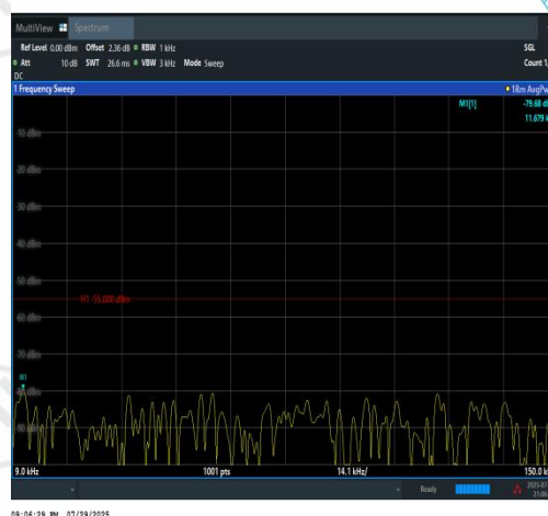
Band7-15MHz-16QAM-21375-75RB#0-0.009~0.15 15-PASS
