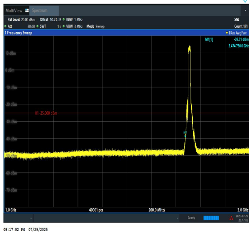
Band7-20MHz-QPSK-20850-100RB#0-1000~30 00-PASS
