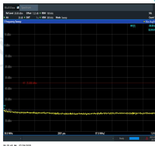
Band7-20MHz-QPSK-21100-1RB#99-30~1000-P
