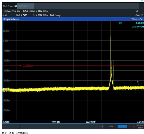
Band7-20MHz-QPSK-21100-1RB#0-1000~3000-PASS
