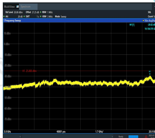
Band7-20MHz-QPSK-21350-100RB#0-3000~20 000-PASS
