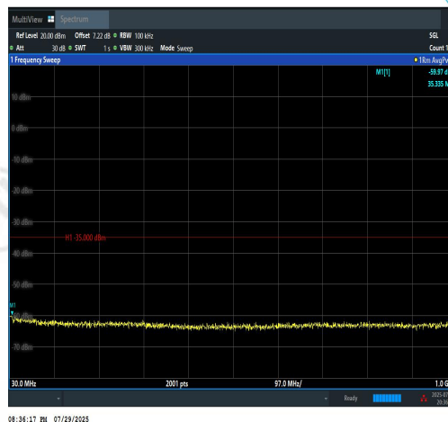
Band7-20MHz-16QAM-21350-1RB#99-30~1000- PASS
