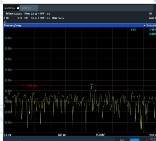
Band7-20MHz-16QAM-21350-1RB#0-0.009~0.1 5-PASS
