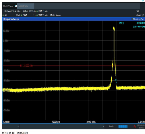
Band7-20MHz-QPSK-21350-100RB#0-1000~30 00-PASS
