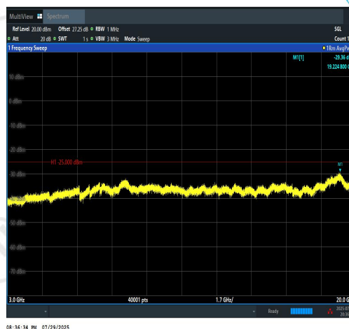
Band7-20MHz-16QAM-21350-1RB#99-3000~20 000-PASS
