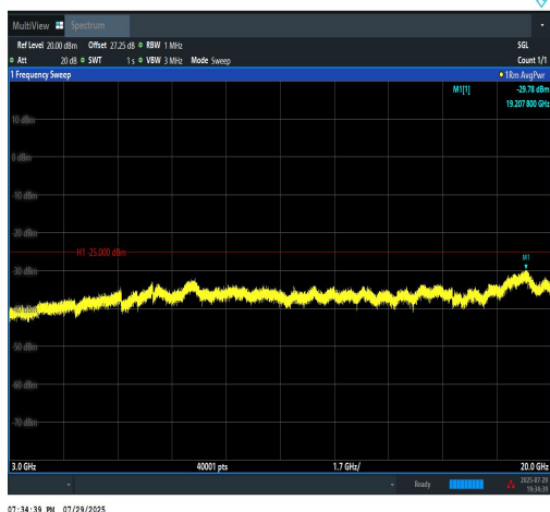
Band7-5MHz-16QAM-20775-25RB#0-3000~200 00-PASS
