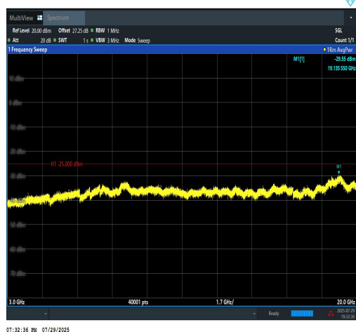
Band7-5MHz-QPSK-20775-1RB#24-3000~2000 0-PASS
