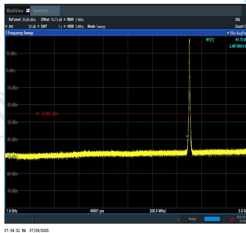
Band7-5MHz-16QAM-20775-25RB#0-1000~300 0-PASS
