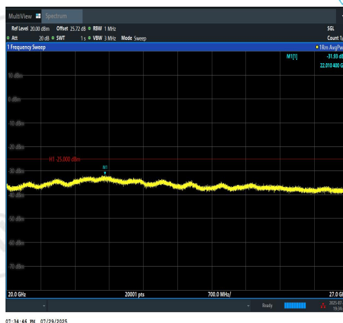
Band7-5MHz-16QAM-20775-25RB#0-20000~27 000-PASS
