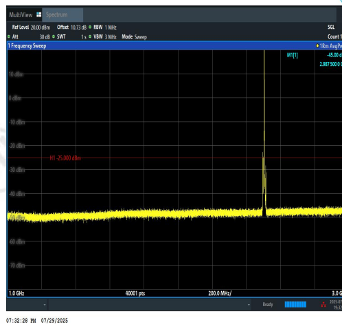
Band7-5MHz-QPSK-20775-1RB#24~3000-PAS S
