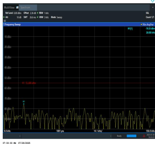
Band7-5MHz-QPSK-20775-25RB#0-0.009~0.15-
