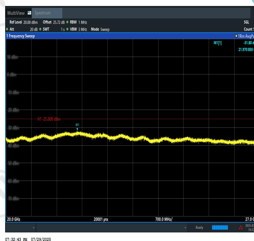
Band7-5MHz-QPSK-20775-1RB#24-20000~270 00-PASS
