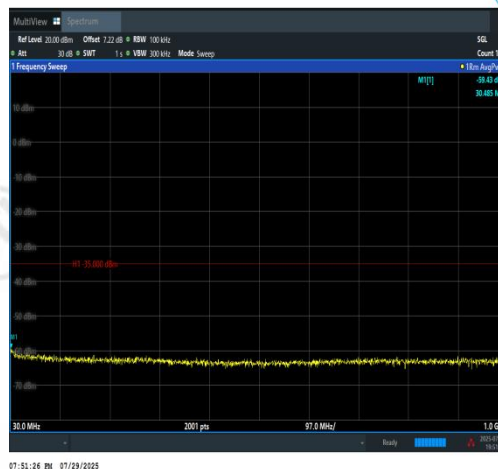
Band7-10MHz-QPSK-21400-1RB#0-30~1000-P
