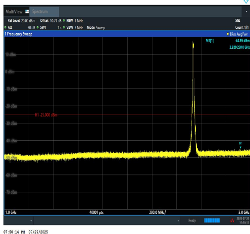
Band7-10MHz-QPSK-21100-50RB#0-1000~300
