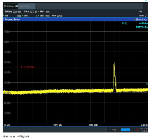
Band7-10MHz-16QAM-21100-1RB#49-1000~30 00-PASS
