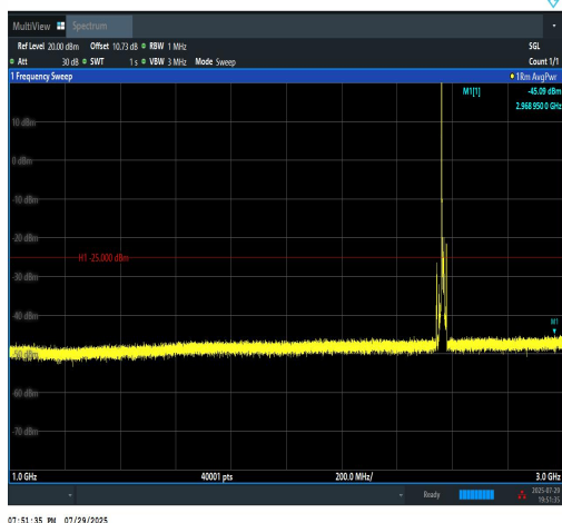
Band7-10MHz-QPSK-21400-1RB#0-1000~3000-
