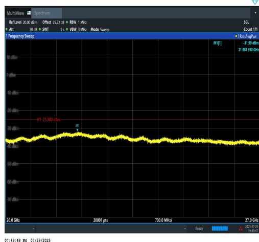
Band7-10MHz-16QAM-21100-1RB#49-20000~2 7000-PASS
