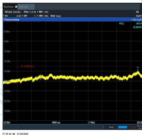
Band7-10MHz-QPSK-21100-50RB#0-3000~200
