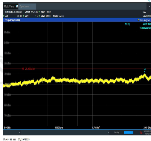
Band7-10MHz-16QAM-21100-1RB#49-3000~20 000-PASS
